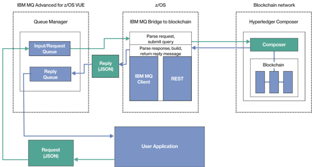
图 99: IBM MQ Bridge to blockchain
