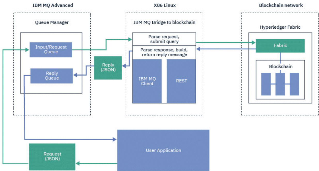
图 98: IBM MQ Bridge to blockchain
