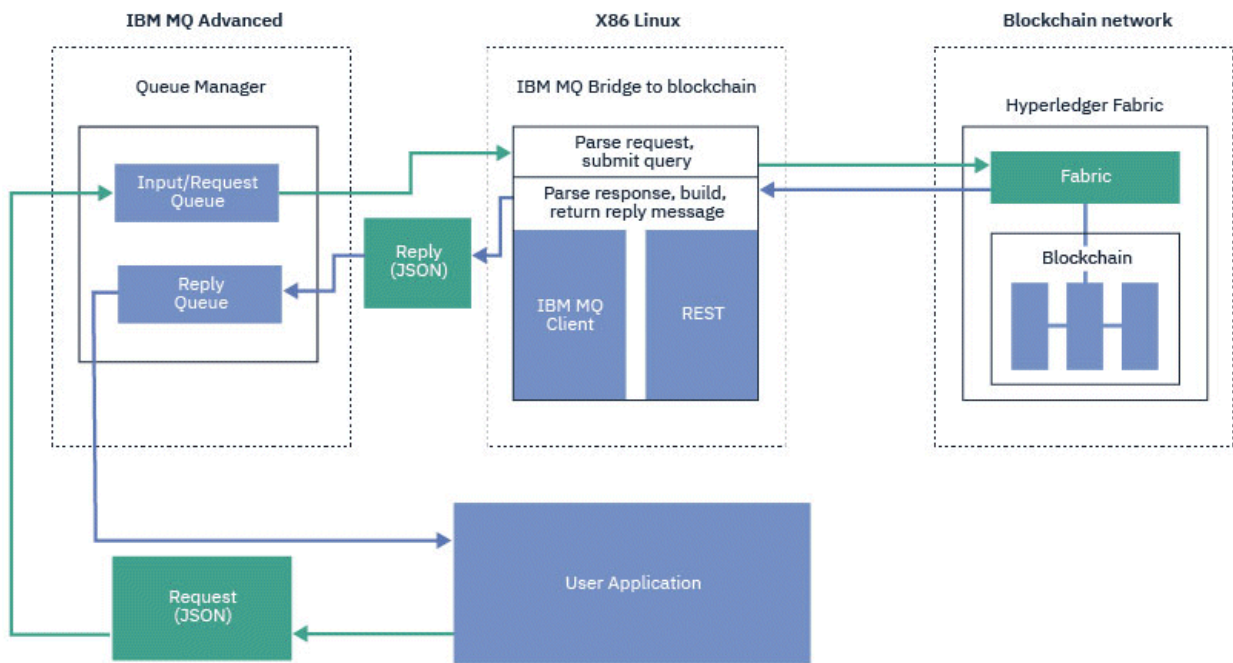
図 98. IBM MQ Bridge to blockchain
