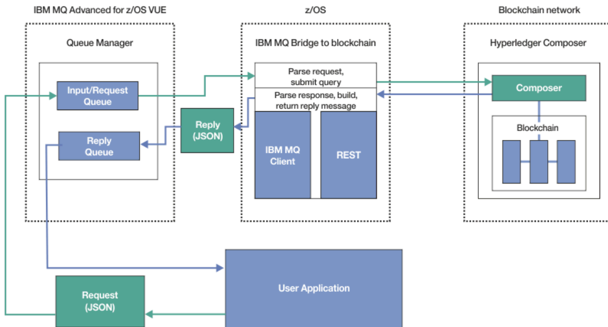
図 99. IBM MQ Bridge to blockchain
