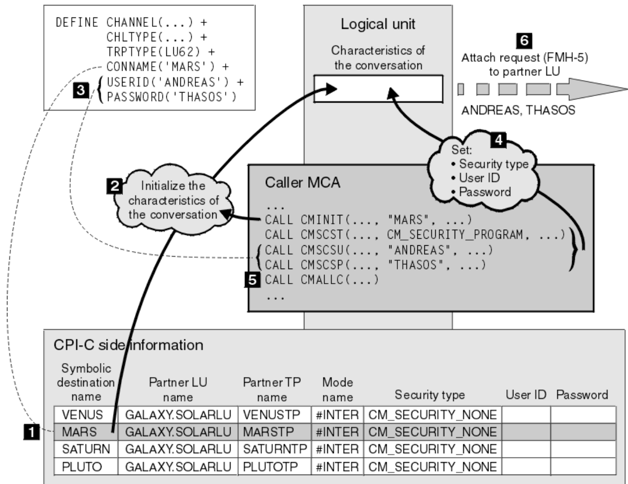
Figure 13. IBM MQ support for conversation level authentication
