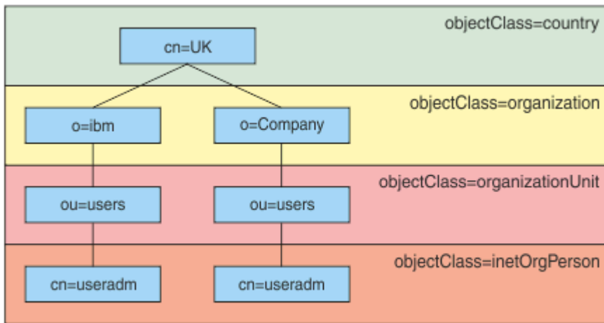
Figure 8. An example LDAP hierarchy
