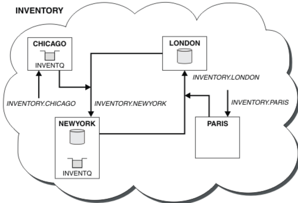
Figure 62. The INVENTORY cluster, with four queue managers
