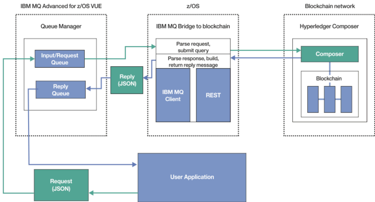
Figure 99. IBM MQ Bridge to blockchain
