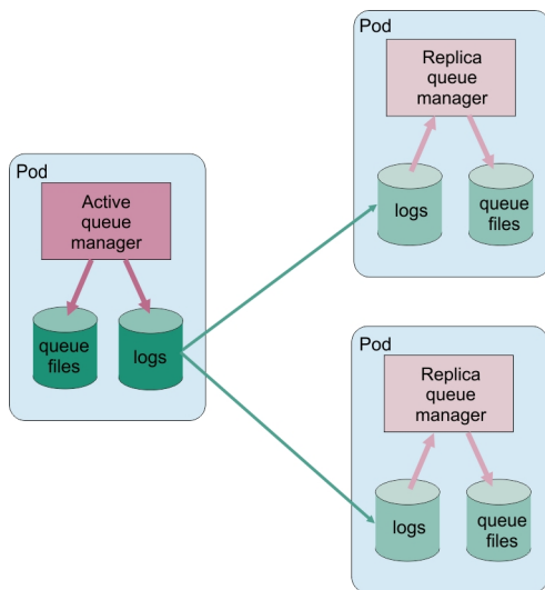
Figure 83. Example of Native HA configuration
