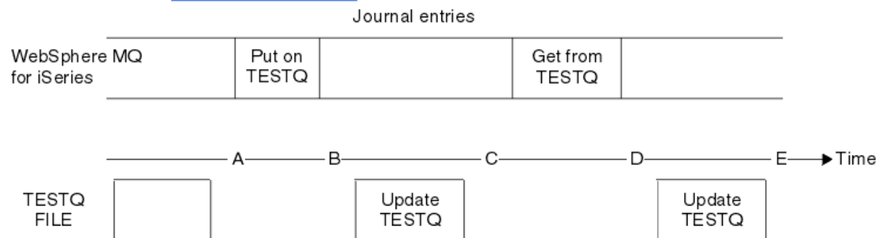
Figure 22. Sequence of events when updating MQM objects
