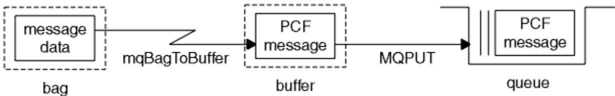
Figure 9. Converting bags to PCF messages
