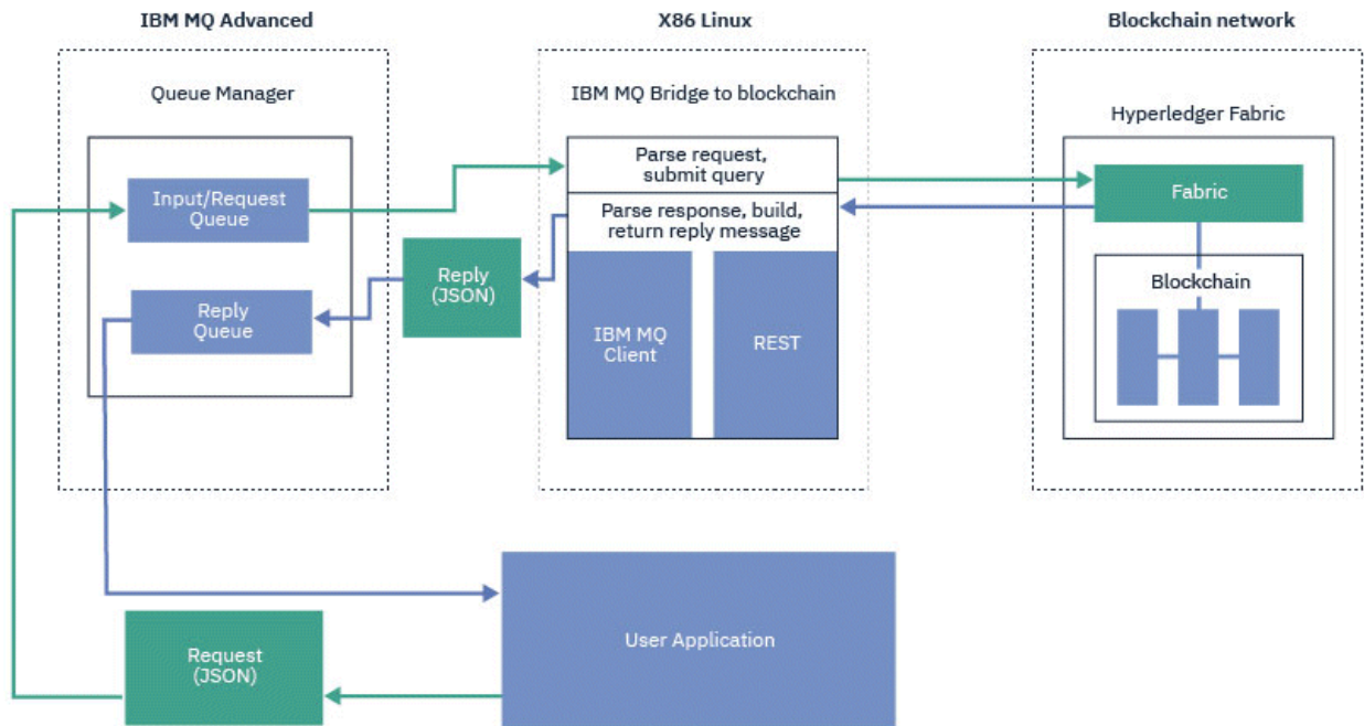
圖 101: IBM MQ Bridge to blockchain
