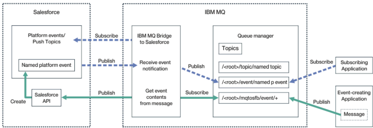
圖 100: IBM MQ Bridge to Salesforce
