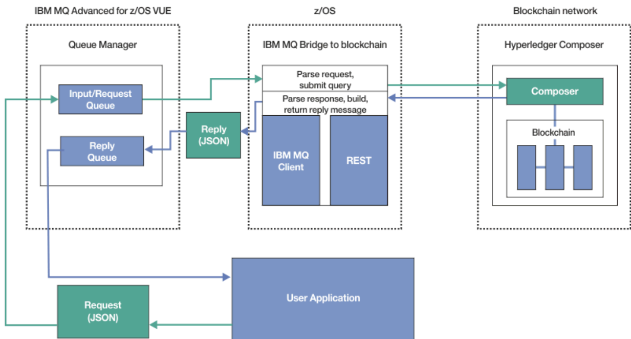
图 128: IBM MQ Bridge to blockchain
