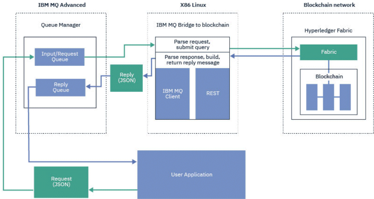
图 101: IBM MQ Bridge to blockchain
