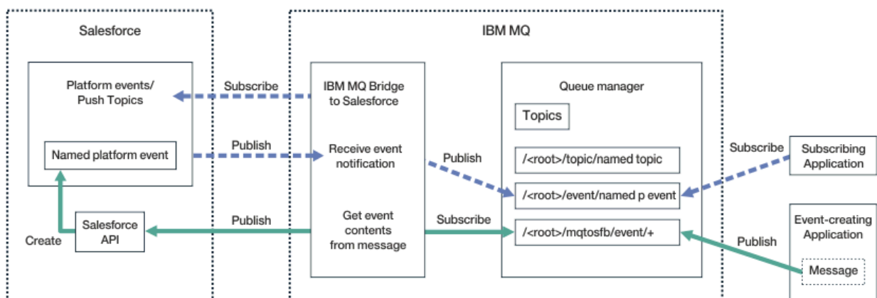
图 100: IBM MQ Bridge to Salesforce
