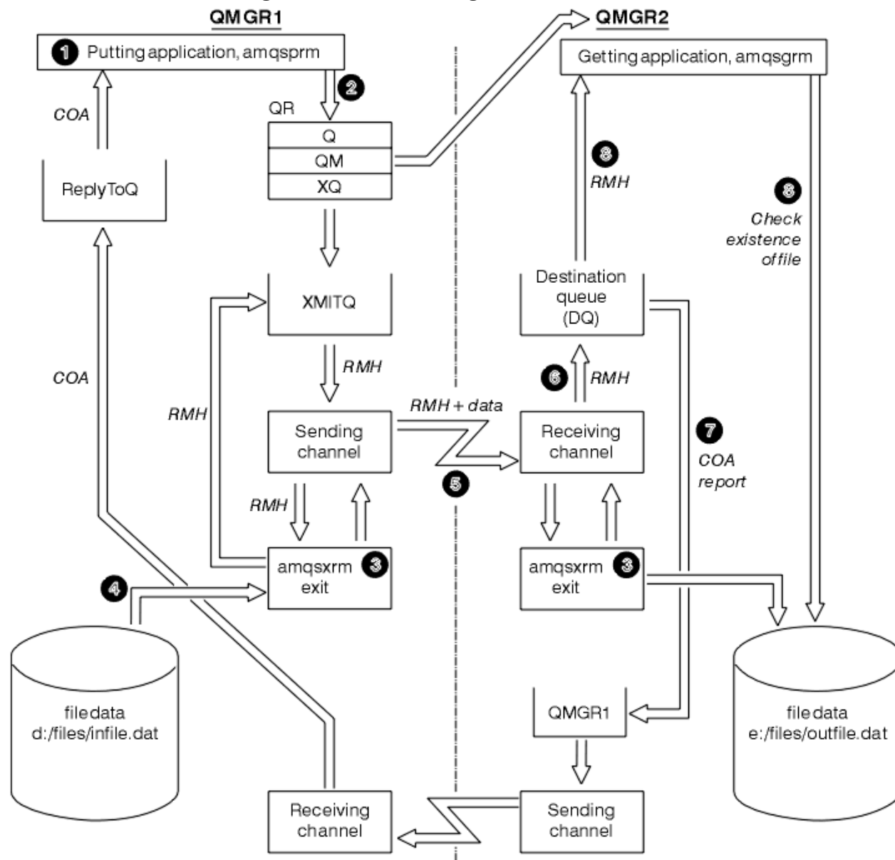
Figura 135. Executando as amostras Reference Message
