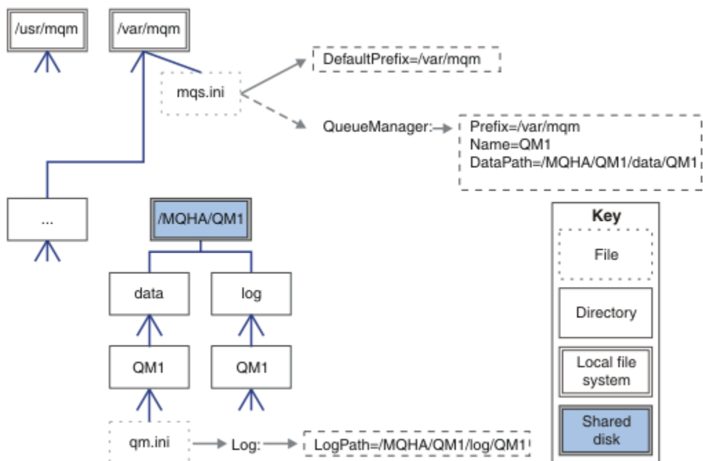
Figura 73. Directory data e log denominate condivise
