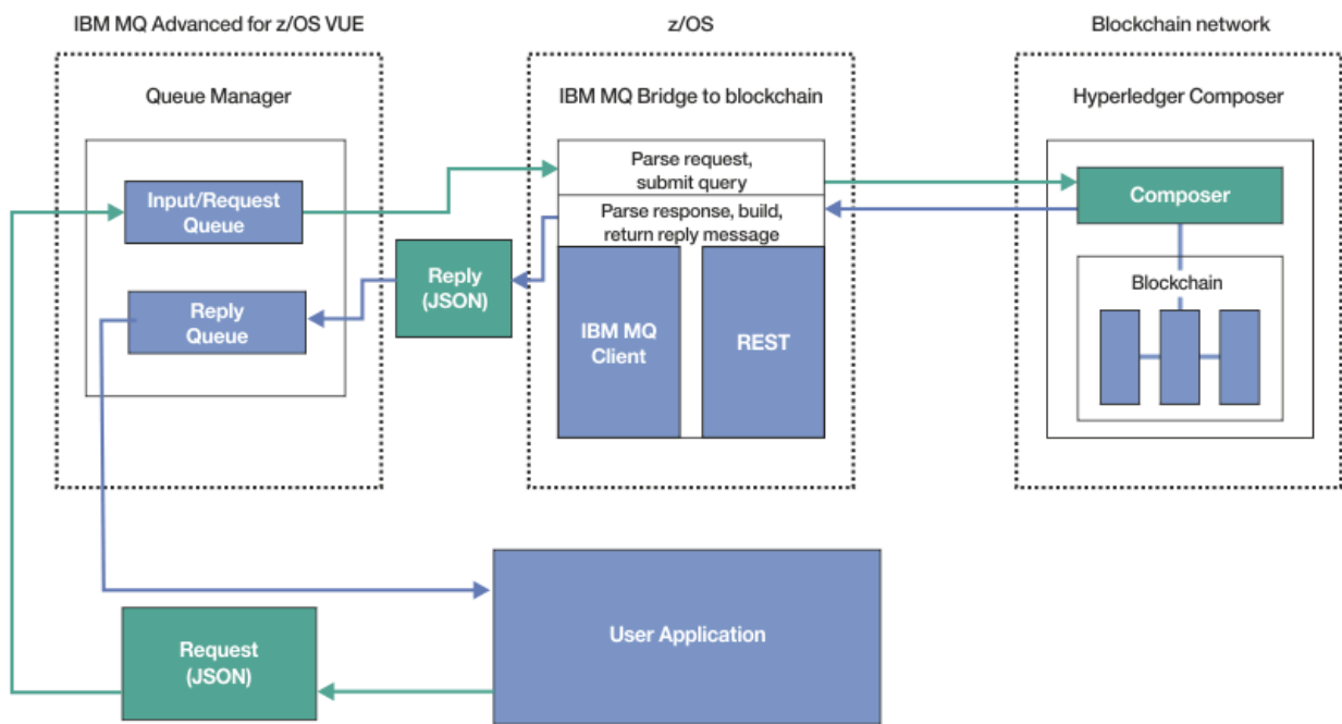
Figura 128. IBM MQ Bridge to blockchain
