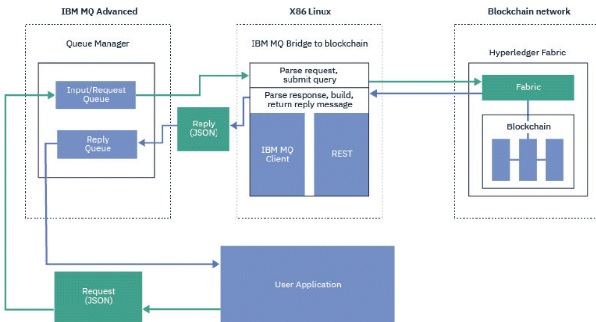
Figura 101. IBM MQ Bridge to blockchain
