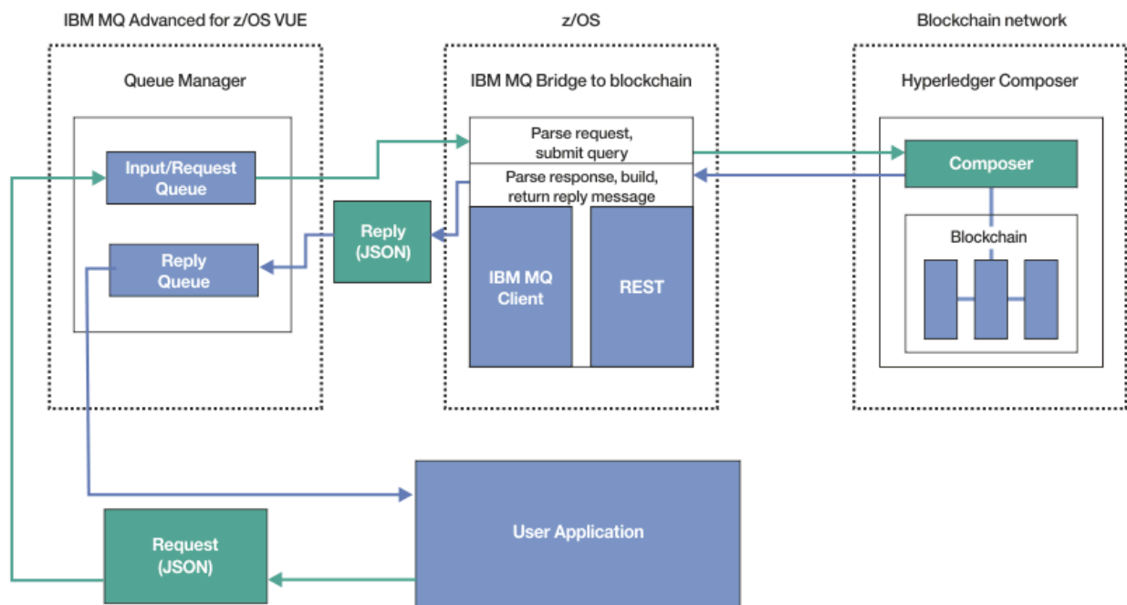
Figura 128. IBM MQ Bridge to blockchain
