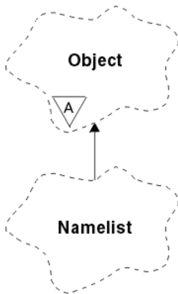
Figure 28. ImqNamelist class
