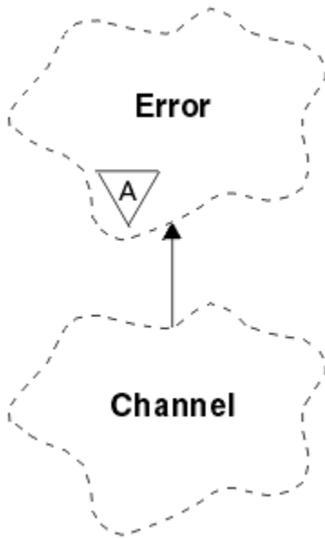
Figure 17. ImqChannel class
