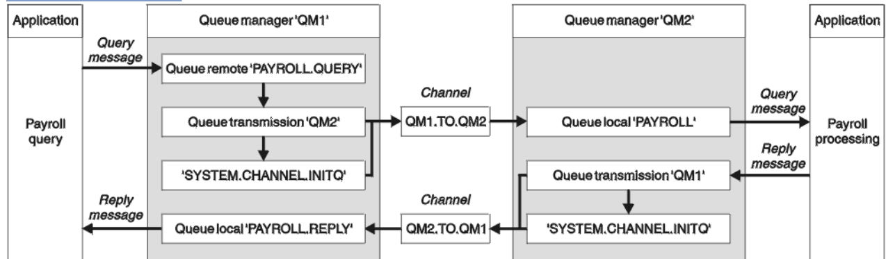
Figure 7. The message channel example for AIX, Linux, and Windows systems
