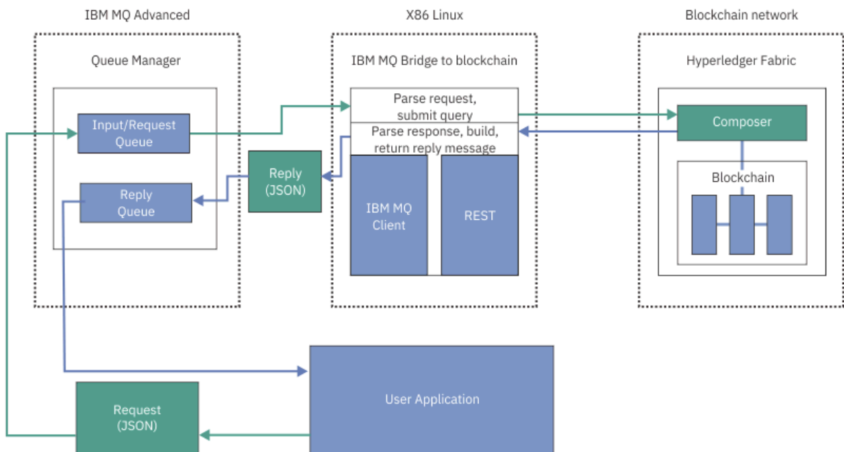
Figure 98. IBM MQ Bridge to blockchain
