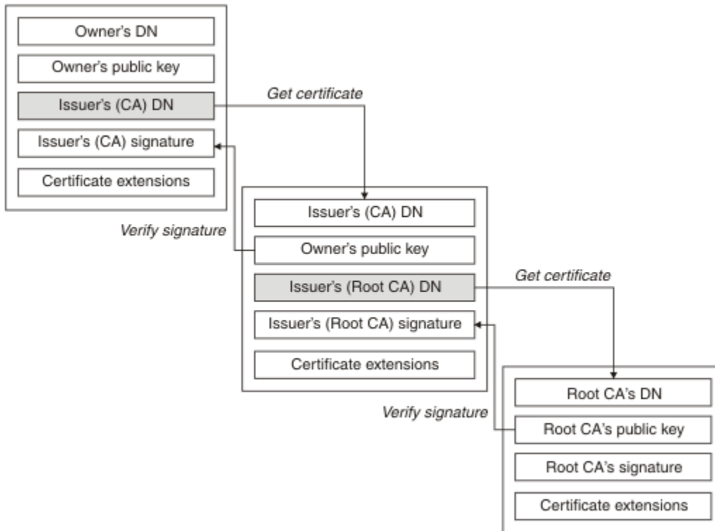
Figure 4. Chain of trust
