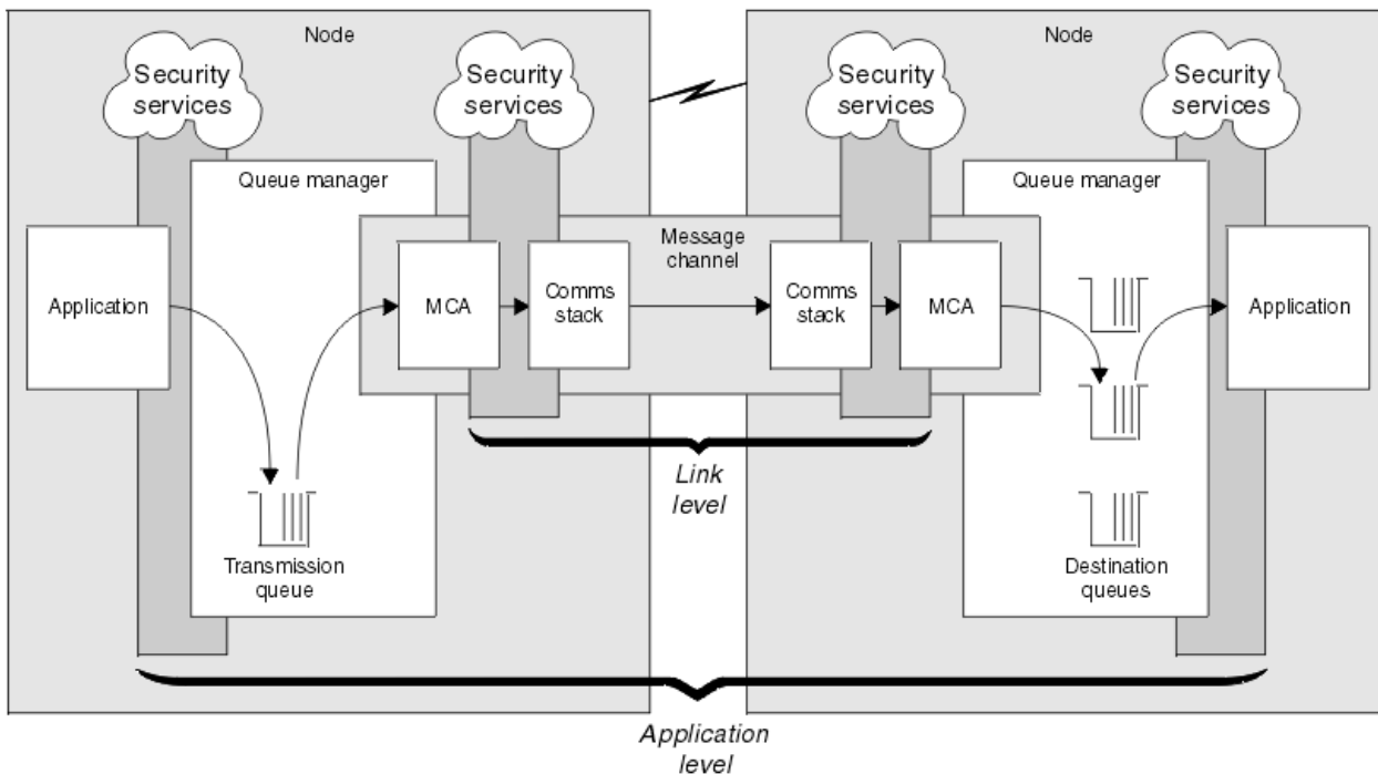
Figure 10. Link level security and application level security
