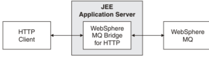
Şekil 200. IBM MQ bridge for HTTP
