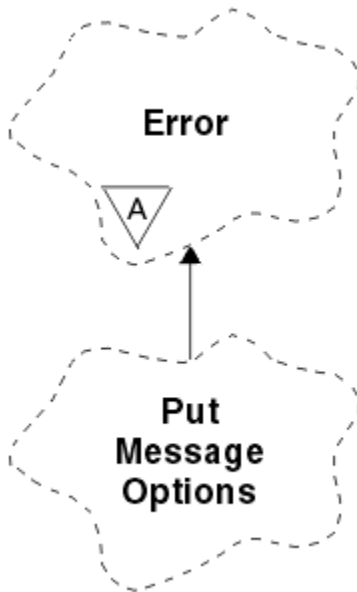
Figure 63. Classe ImqPutMessageOptions
