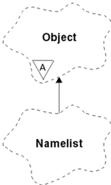
Figure 60. Classe ImqNamelist
