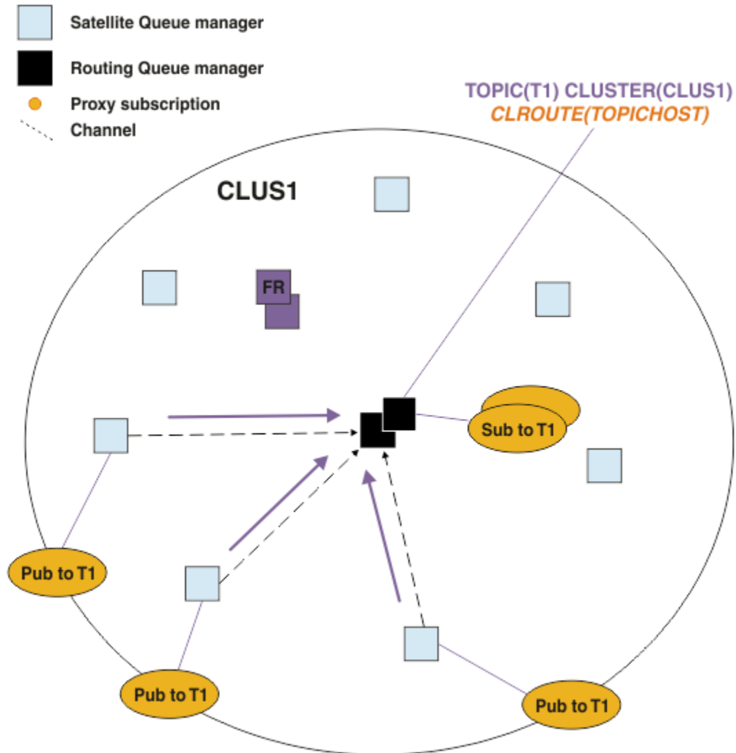
Figure 27. Hosting subscriptions on a topic host queue manager
