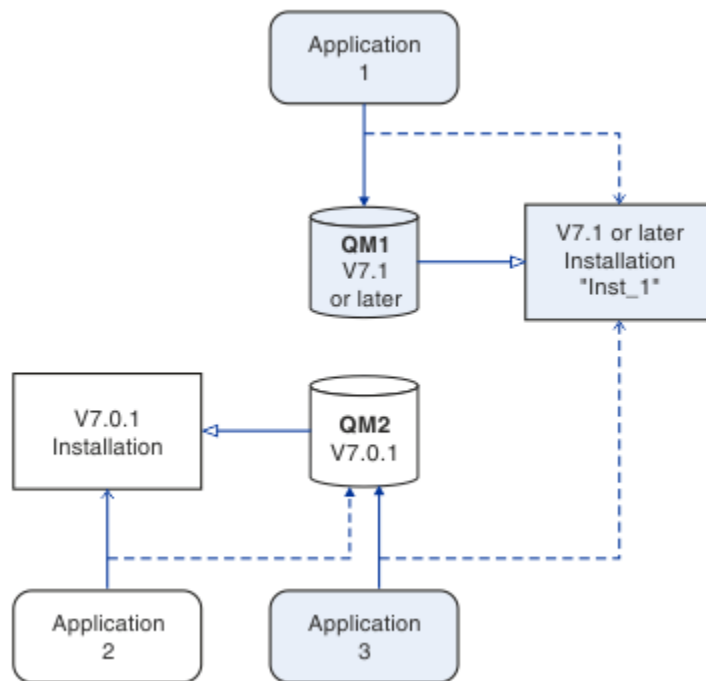
Figure 5. Coexistence of two queue managers using Version 7.0.1 and a later version installations
