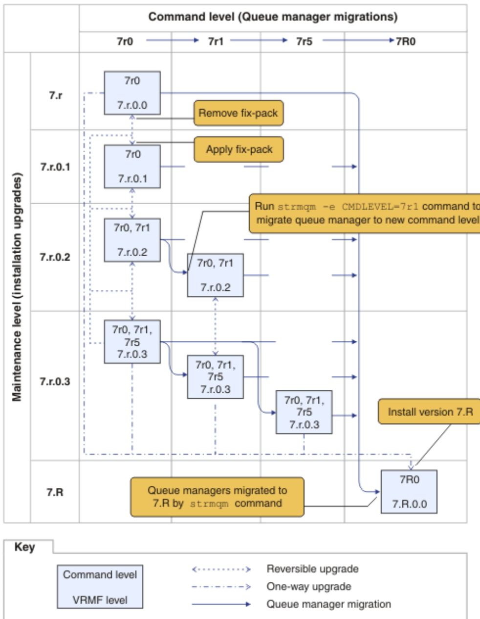
Figure 14. Migration of queue managers to new command levels using new-function fix packs
