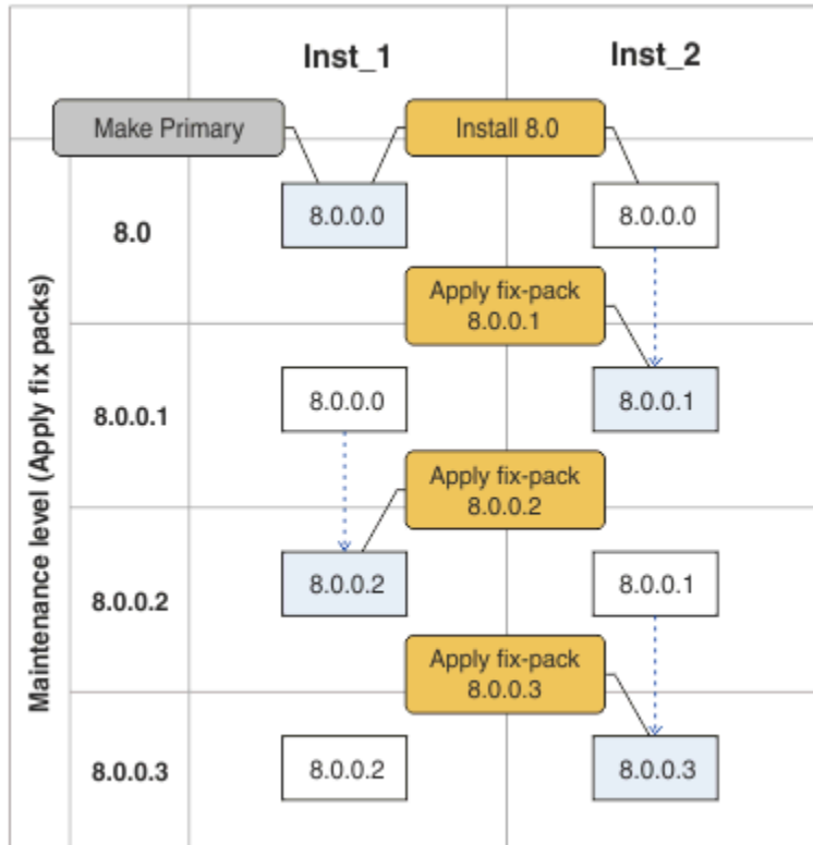
Figure 20. Rolling fix releases
