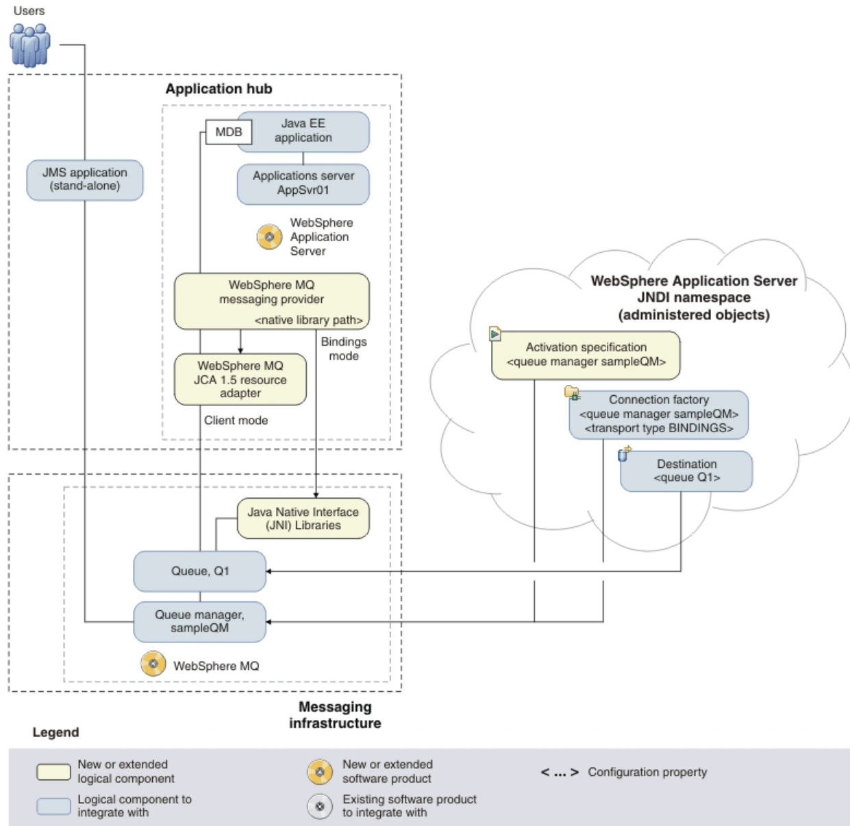
Figure 9. Delivered logical topology. The high-level logical topology diagram for software functions delivered by migrating WebSphere Application Server and WebSphere MQ from Version 6 to Version 7. This logical topology shows the new functions as new or extended logical components, integrated with the software functions and products from the initial logical topology.
