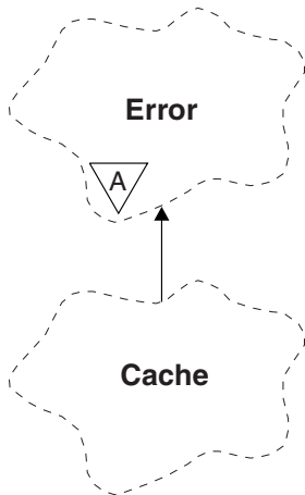
Figure 5. ImqCache class
