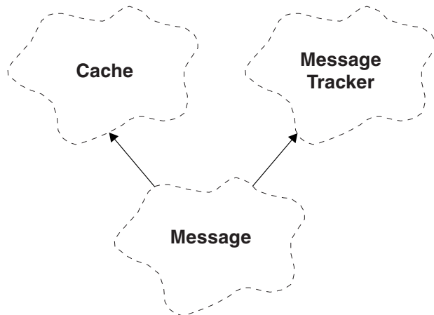
Figure 15. ImqMessage class
