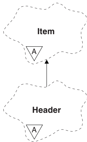
Figure 12. ImqHeader class
