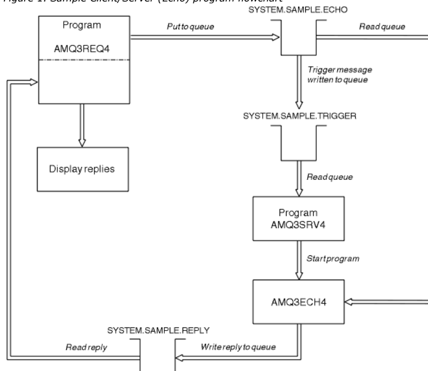
Figure 1. Sample Client/Server (Echo) program flowchart
