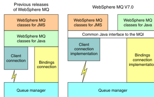
Figure 2. The relationship between WebSphere MQ classes for JMS and WebSphere MQ classes for Java
