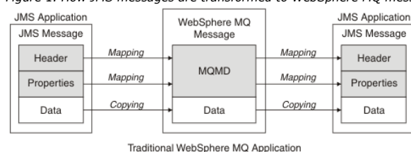
Figure 1. How JMS messages are transformed to WebSphere MQ messages with no MQRFH2 header
