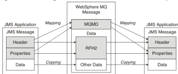
Figure 1. How messages are transformed between JMS and WebSphere MQ using the MQRFH2 header
