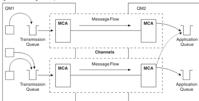
Figure 1. Using multiple channels
