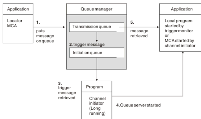
Figure 1. The concepts of triggering
