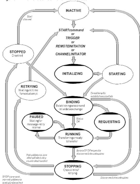
Figure 1. Flows between channel states
