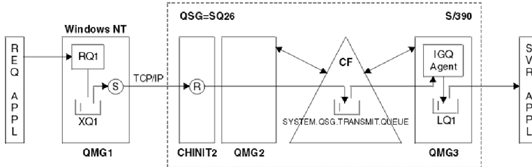
Figure 1. An example of migration support
