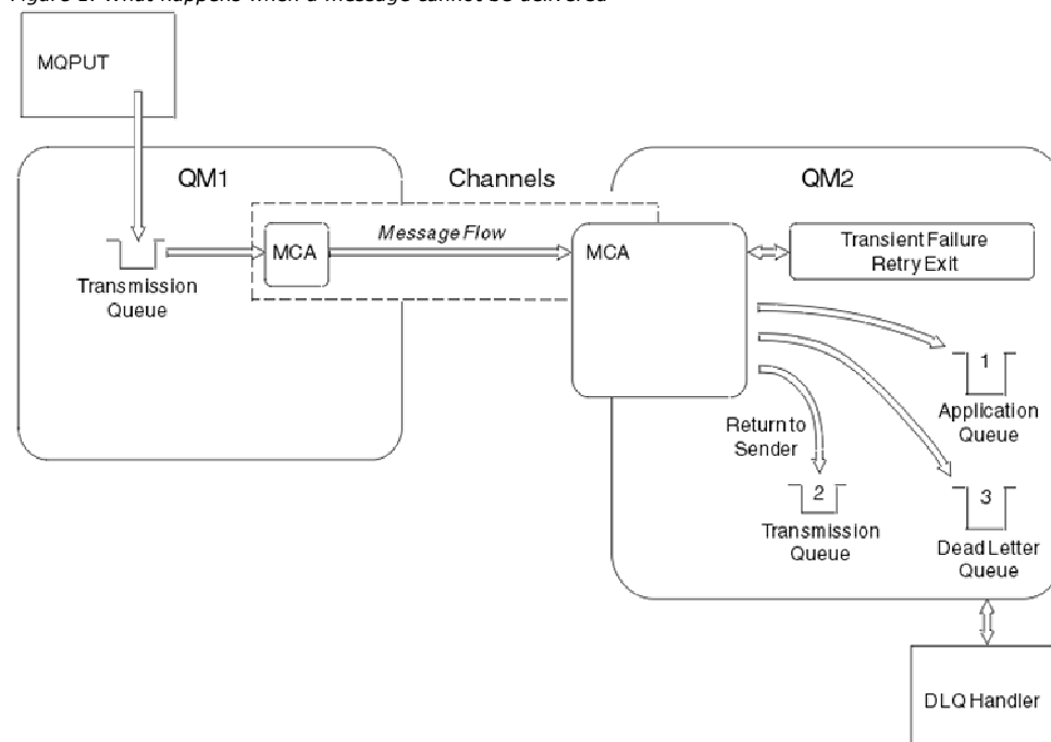
Figure 1. What happens when a message cannot be delivered
