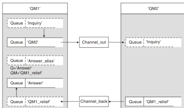
Figure 1. Reply-to queue alias example
