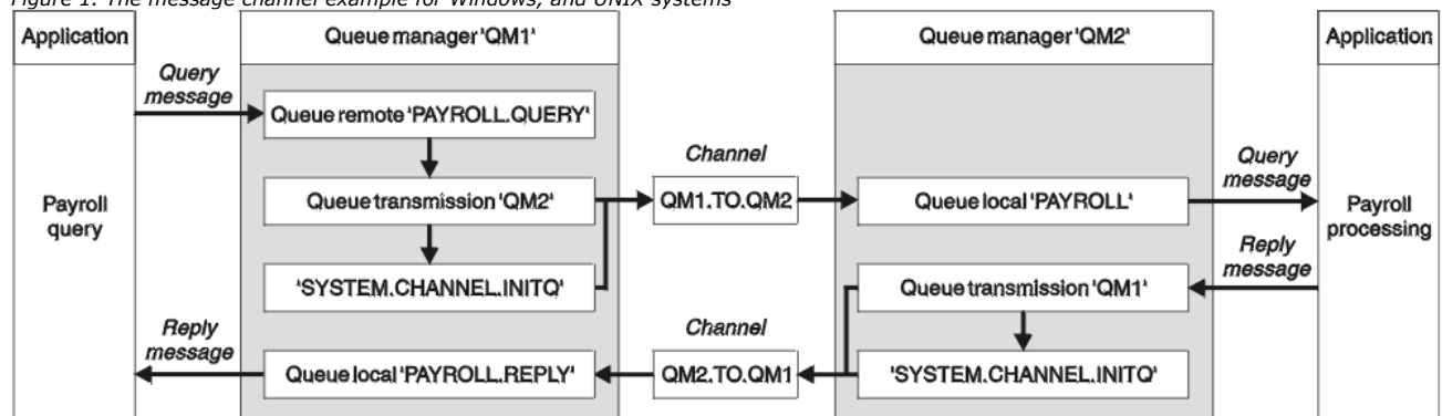
Figure 1. The message channel example for Windows, and UNIX systems
