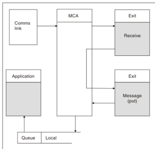
Figure 3. Example of a receive exit at the receiver end of message channel
