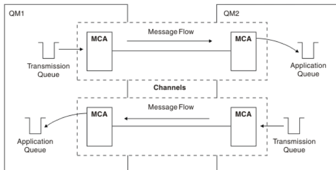
Figure 1. Sending messages in both directions
