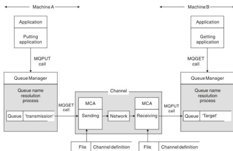
Figure 1. Name resolution
