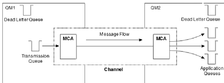
Figure 1. Sending messages
