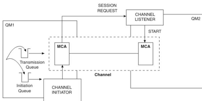
Figure 1. Channel initiators and listeners
