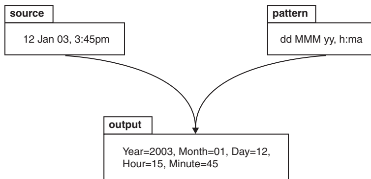
Figure 4. Using a pattern to parse a string source to produce a dateTime output.
