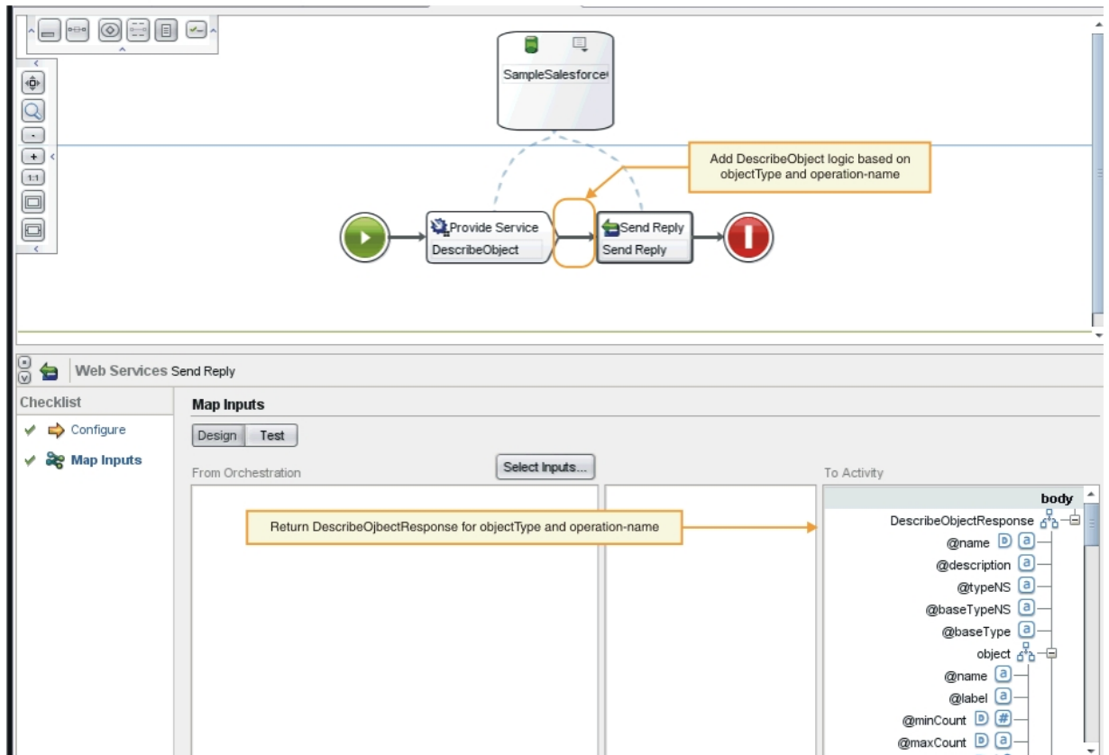
图 1. DescribeObjects
