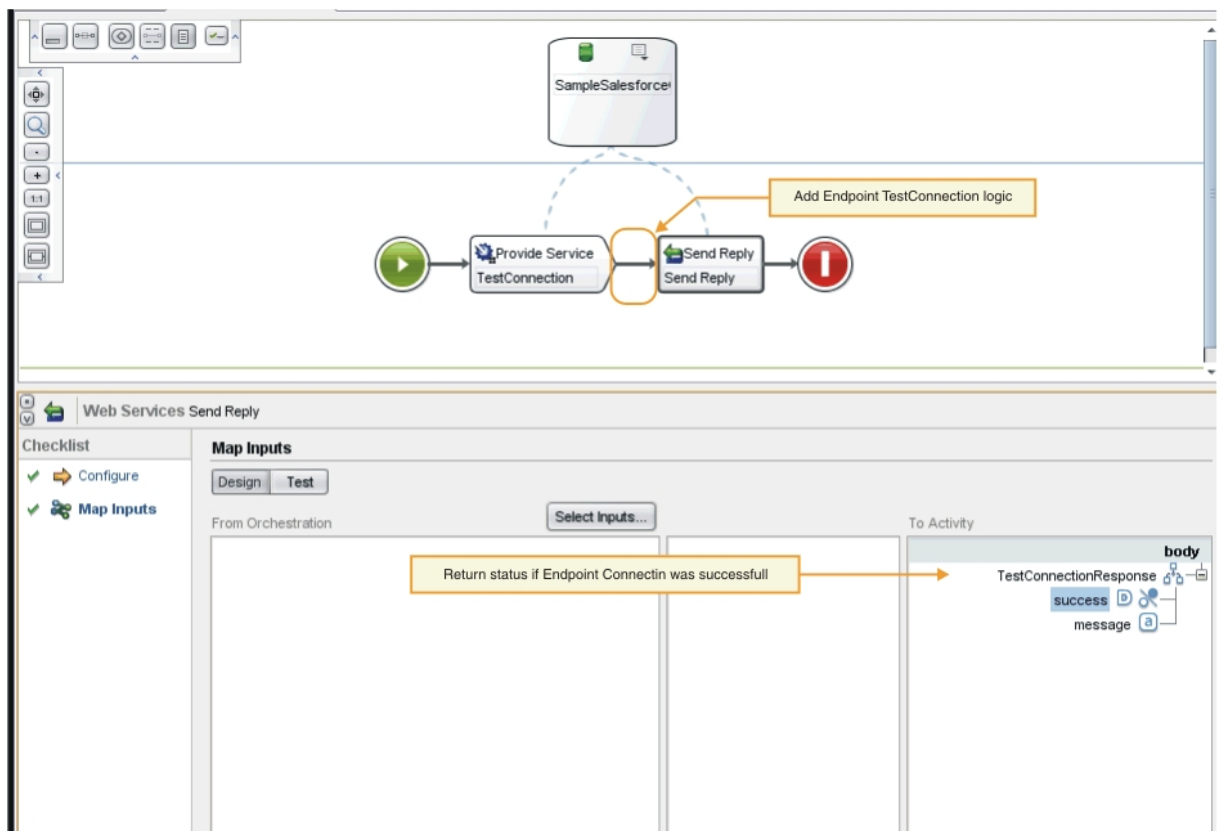
Figura 1. TestConnection
