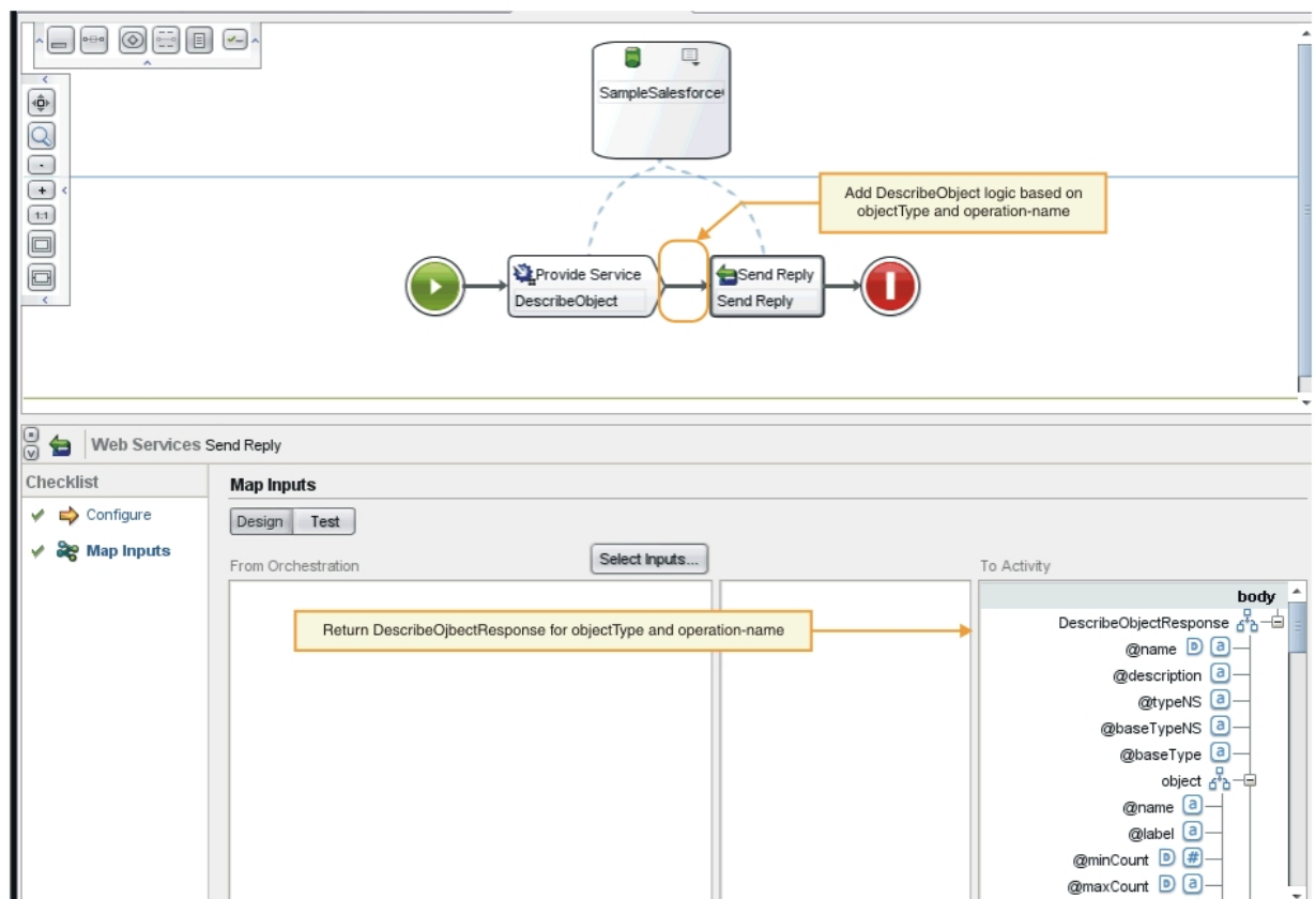
Figura 1. DescribeObjects
