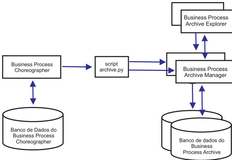
Figura 9. Business Process Choreographer usando dois Business Process Archives
