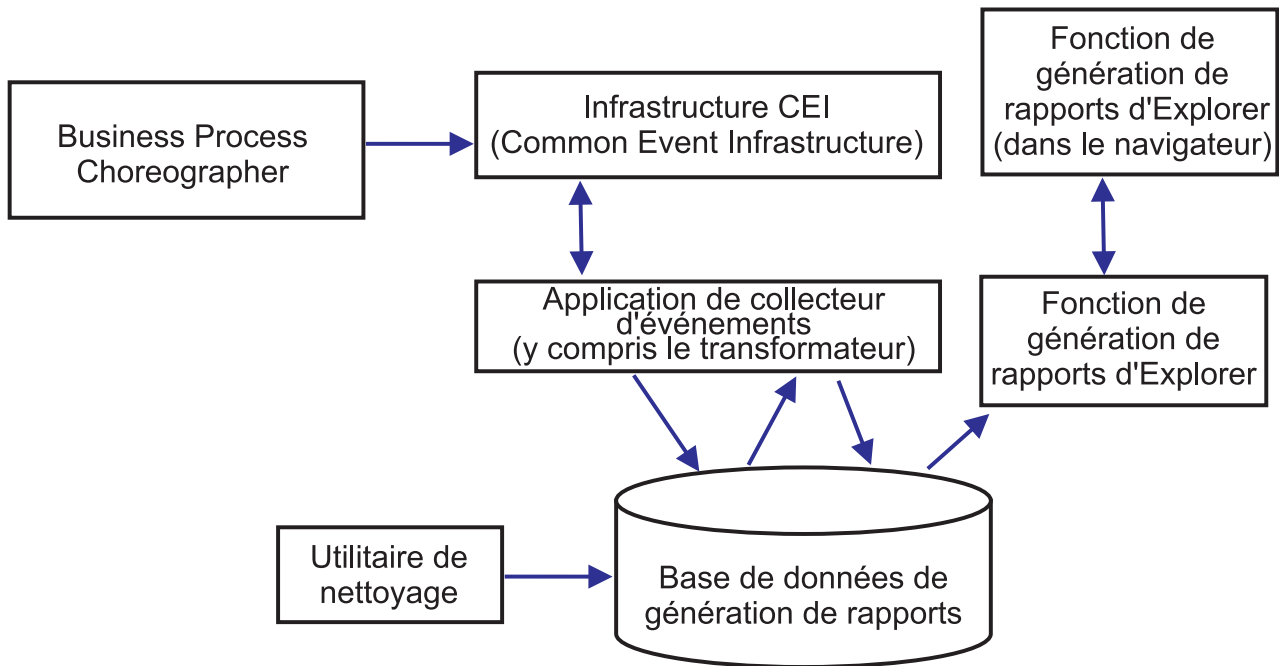
Figure 8. Architecture
