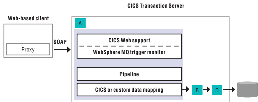
Figure 5. Web services capabilities are now fully integrated into CICS Transaction Server, Version 3.
