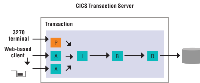
Figure 4. Access options provided by CICS facilitate effective reuse of existing business logic.
