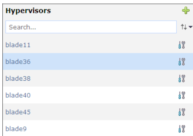
Figure 5-37 Hypervisors' list
