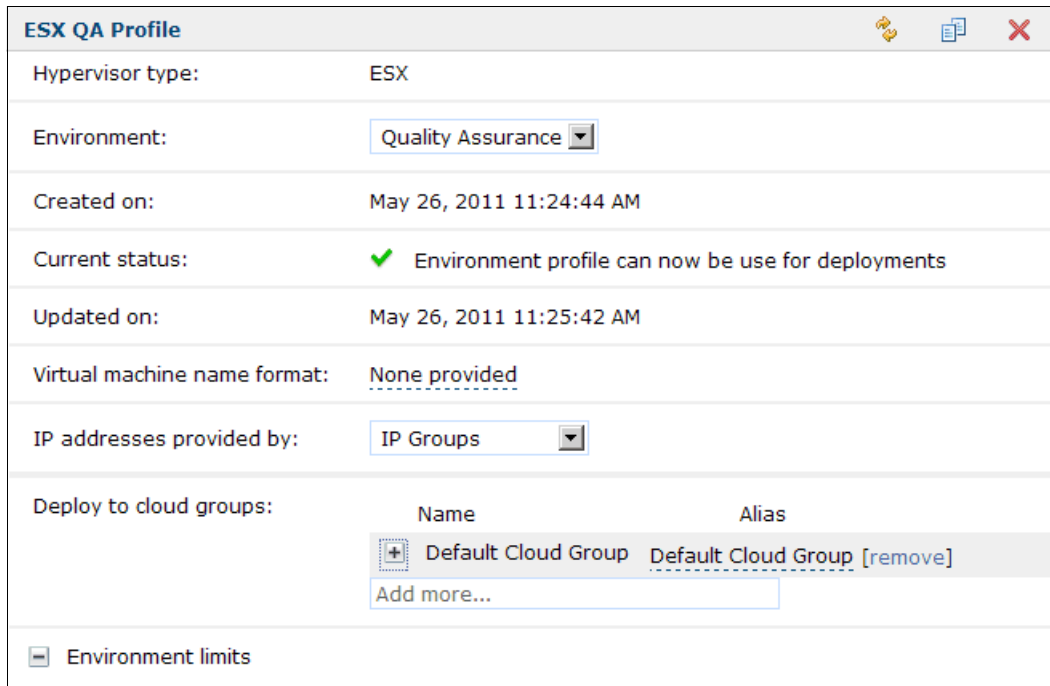
Figure 2-8 Managing environment profiles on IBM Workload Deployer
