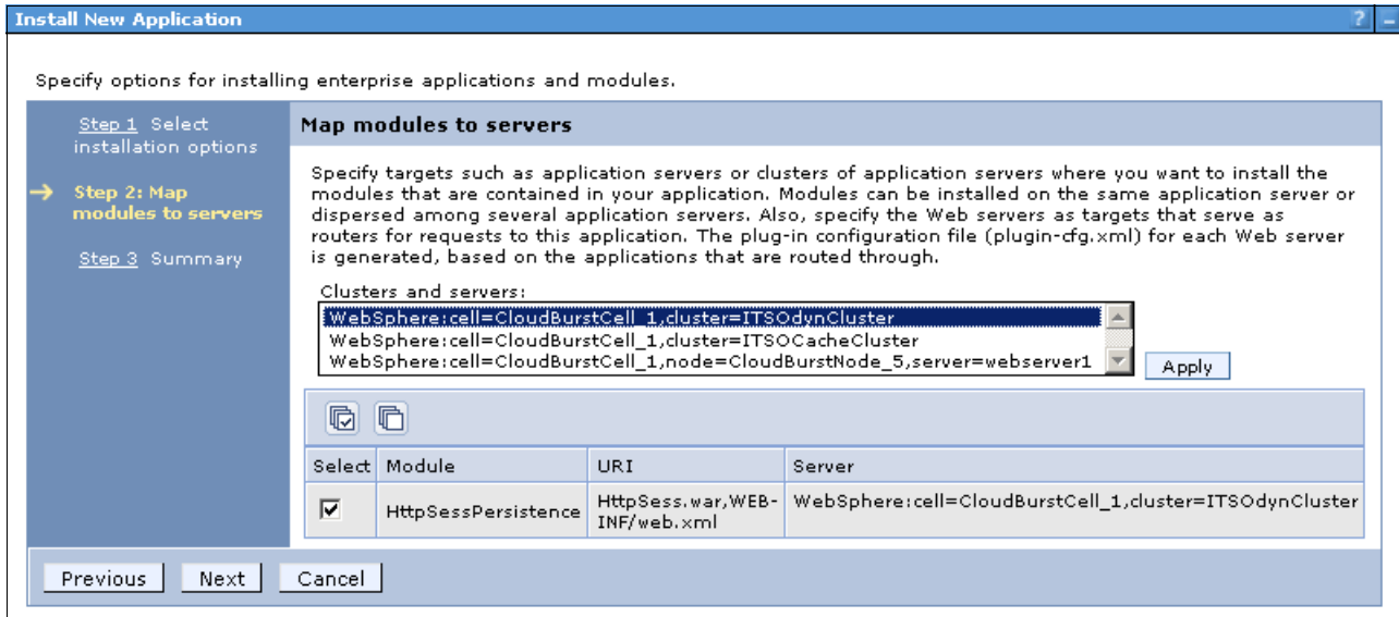
Figure 8-56 Map the application on the dynamic cluster
