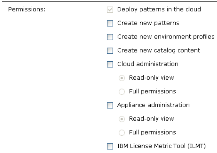
Figure 5-19 ITSOadm1 permissions
