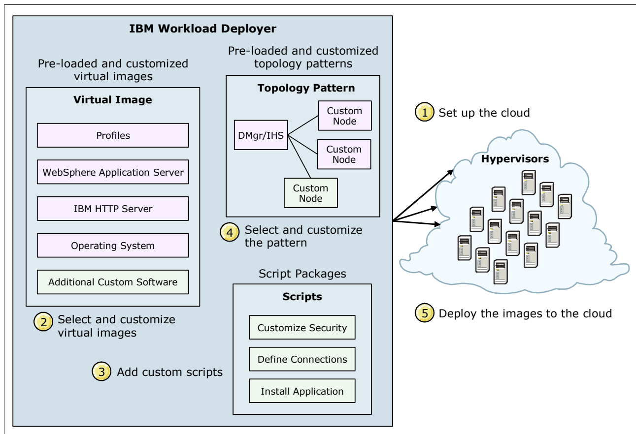
Figure 2-2 IBM Workload Deployer technology preview
