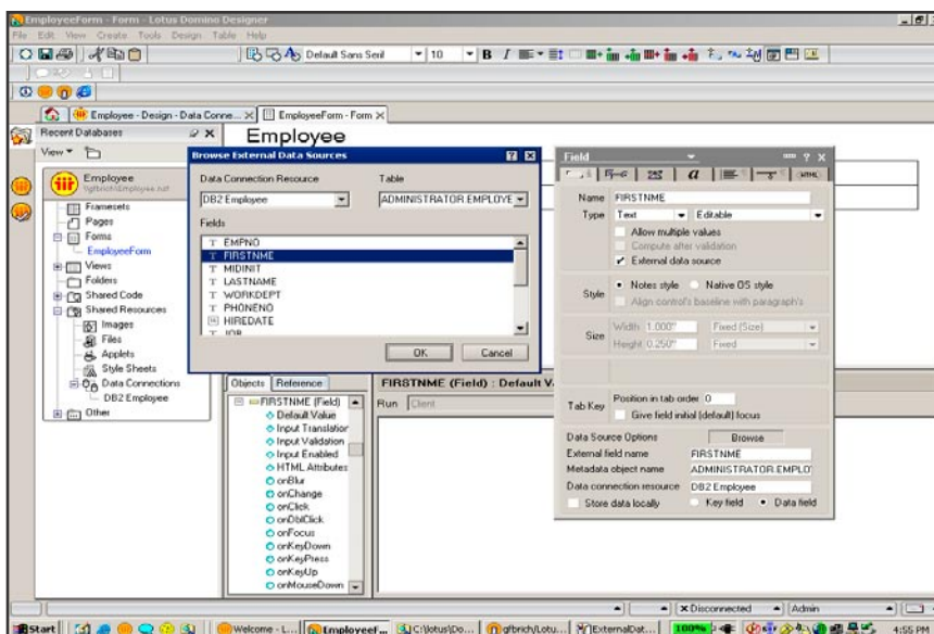
You can use Lotus Domino enterprise connection services and DCRs to map a field in a Lotus Domino form to a column in a DB2 table.
