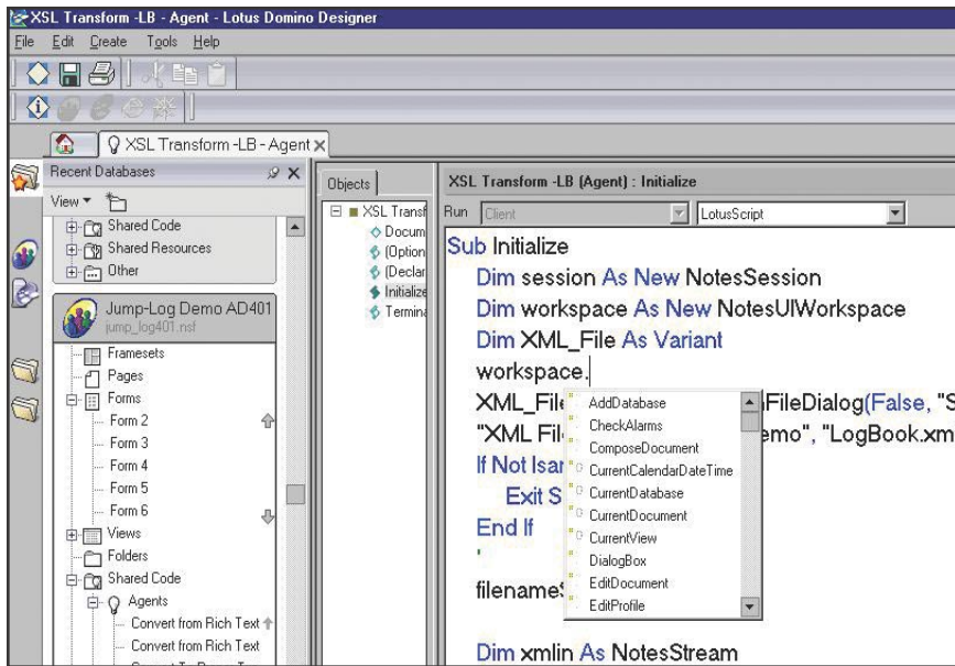
Lotus Domino Designer 6.5 software offers new database navigation and automatic completion of LotusScript code.
