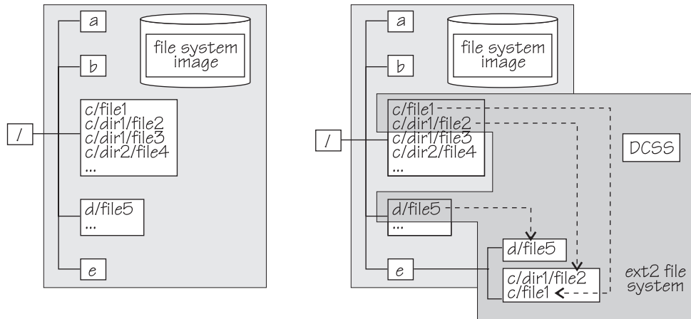
Figure 6. ext2 with the xip mount option over-mounting individual files
