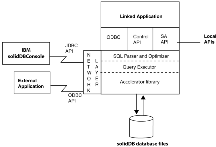
Figure 2.3. IBM solidDB with Linked Library Access - APIs
