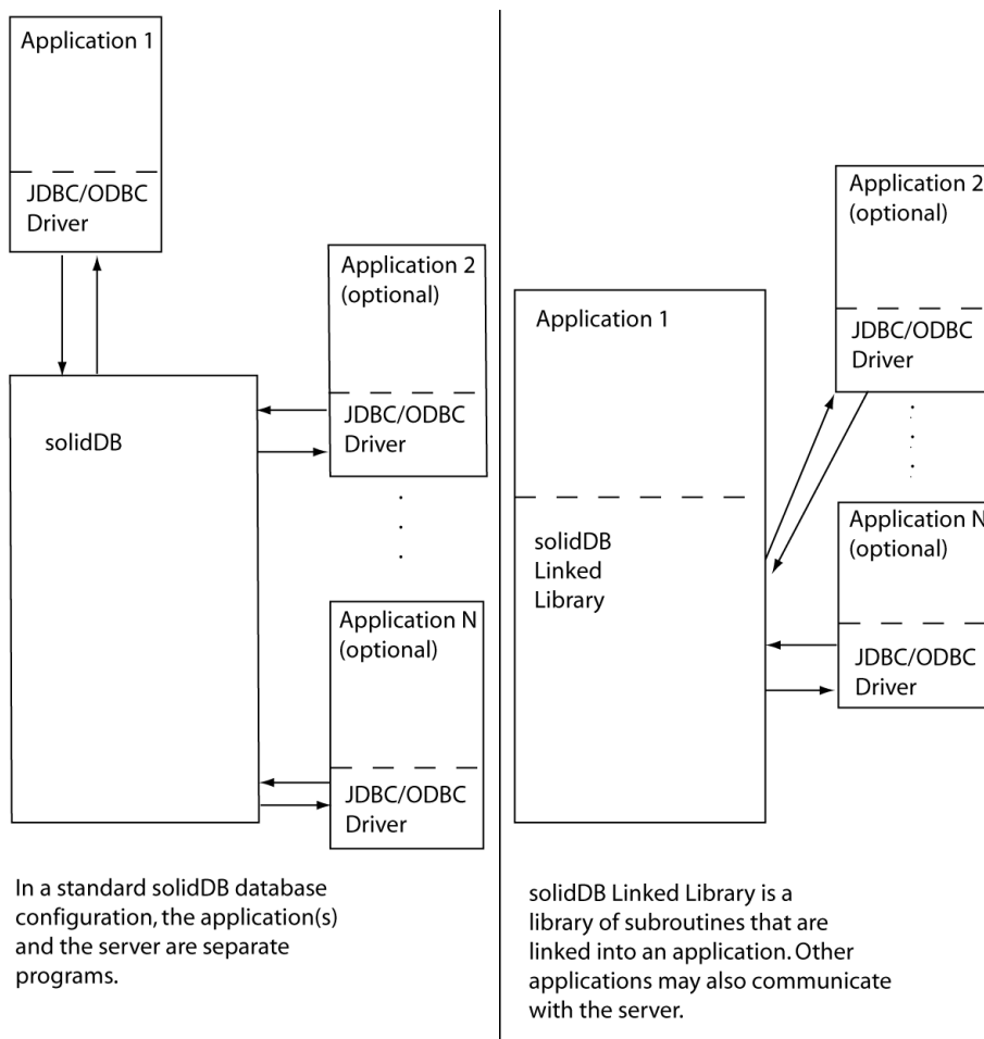
Figure 2.1. IBM solidDB with Linked Library Access
