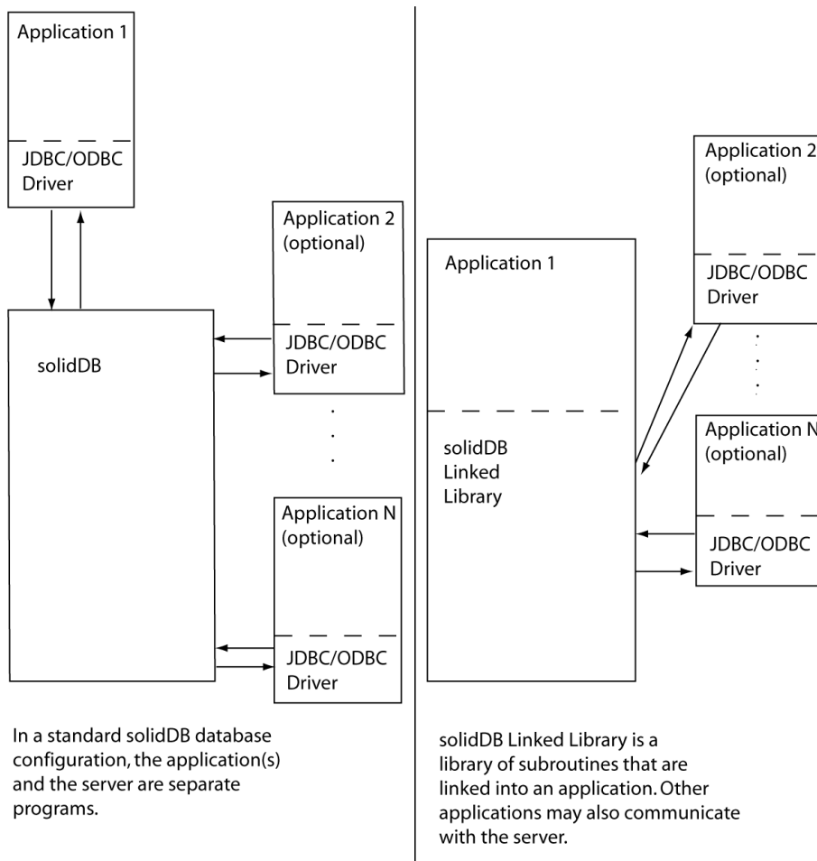
Figure 2.2. Linking to IBM solidDB
