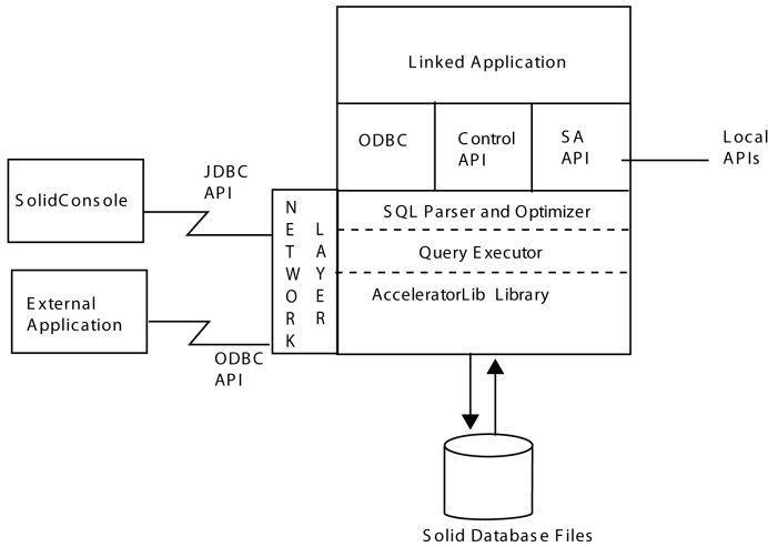
Figure 2.3. solidDB with AcceleratorLib - APIs
