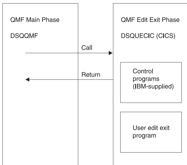
Figure 217. How a governor exit routine works with QMF for VSE
