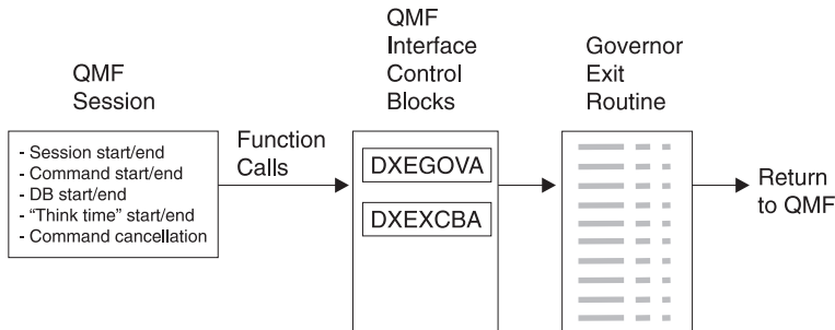
Figure 202. How a governor exit routine works with QMF CMS
