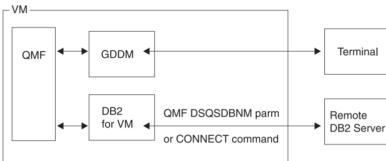
Figure 32. QMF Relationship to VM, DB2 for VM, and GDDM
