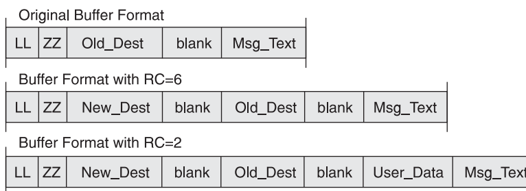
Figure 32. Old and New Buffer Formats
