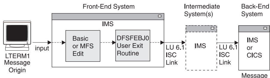
Figure 30. Message Flow with the Front-End Switch Exit Routine
