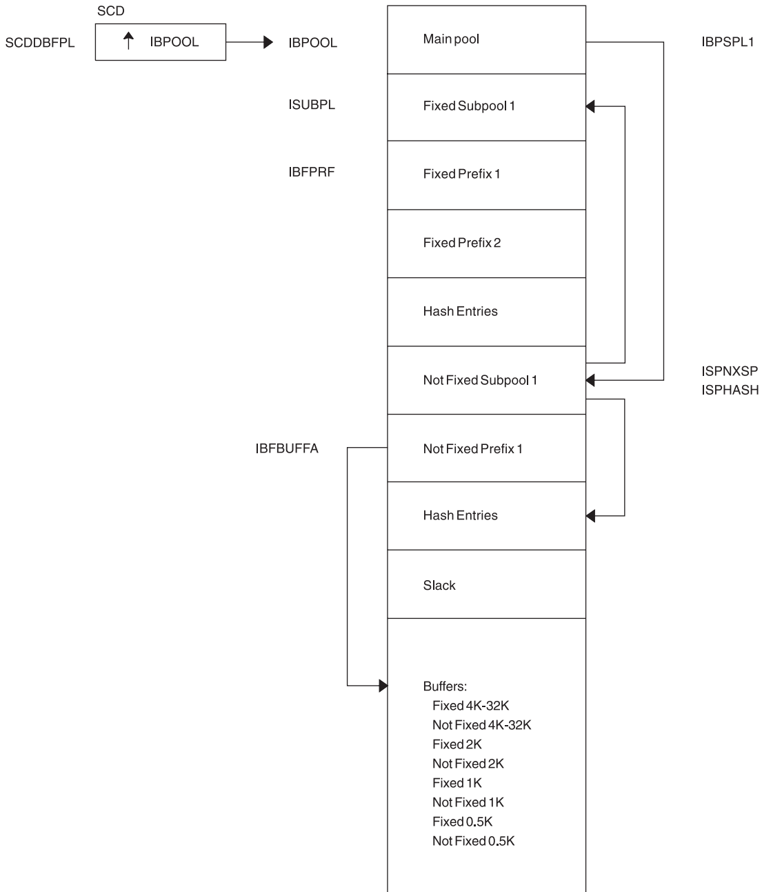
Figure 4. DL/I Buffer Pool (OSAM and VSAM)
