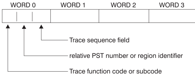
Figure 61. General Trace Record Format
