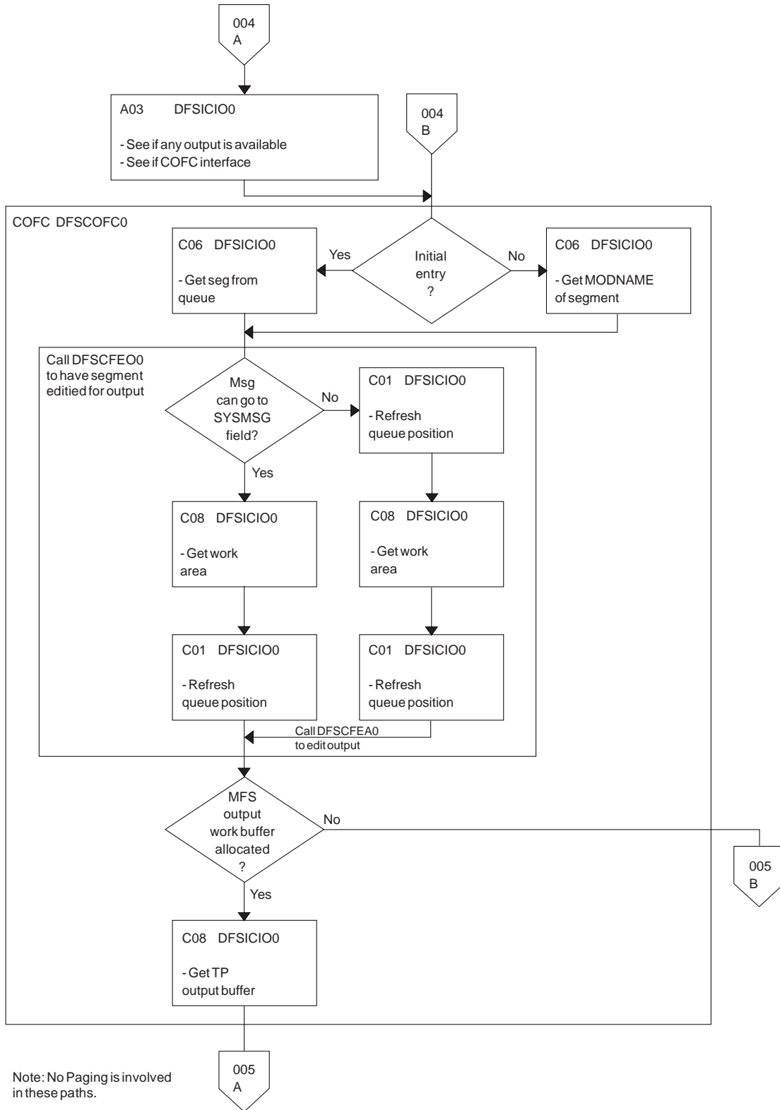
Figure 135. Message Format Service (MFS) Normal BTAM Path (Part 4 of 5)
