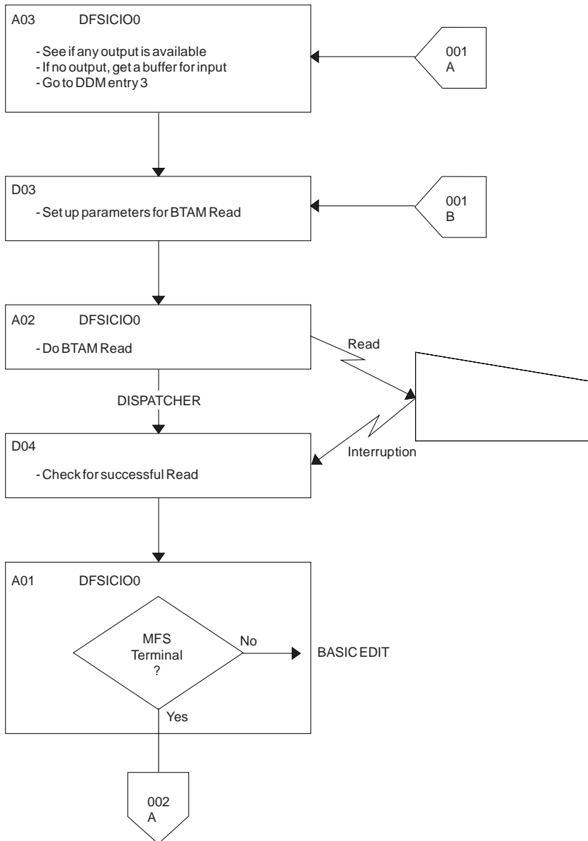
Figure 135. Message Format Service (MFS) Normal BTAM Path (Part 1 of 5)
