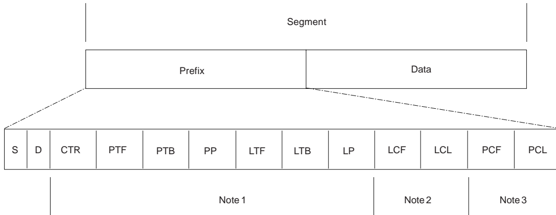
Figure 37. Mapping the Prefix of a Segment
