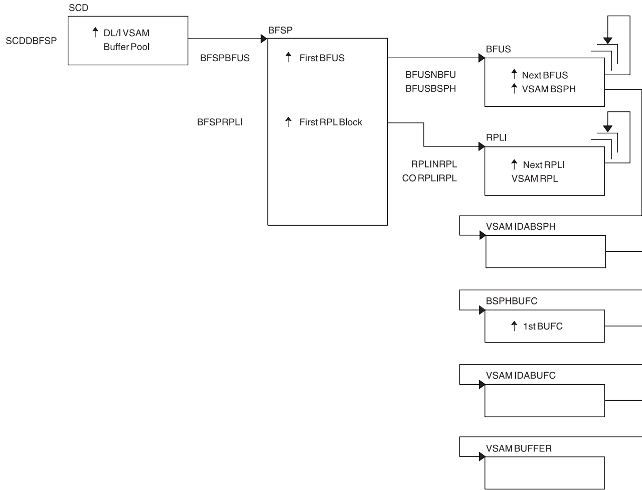
Figure 6. Buffer Handler Pool (VSAM)
