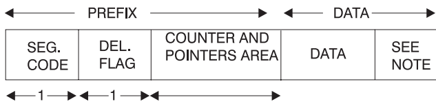
Figure 36. HDAM, HIDAM, PHDAM, or PHIDAM Segment Format
