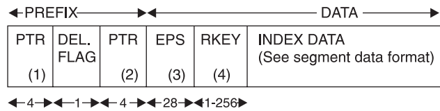
Figure 39. LRECL Format on Device and in Buffer Pool
