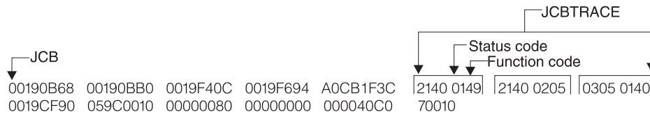
Figure 82. Example of a Job Control Block (JCB) Dump
