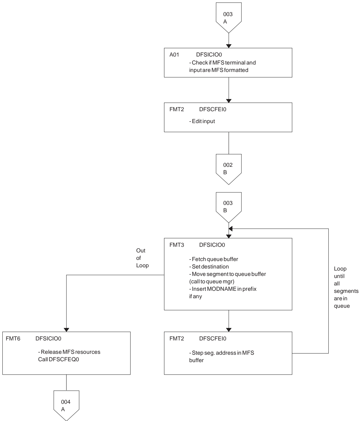
Figure 135. Message Format Service (MFS) Normal BTAM Path (Part 3 of 5)
