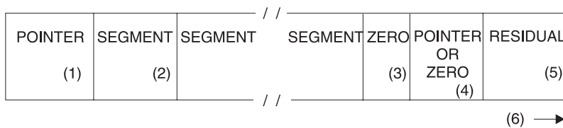
Figure 35. LRECL Format
