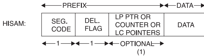
Figure 34. HISAM Segment Format
