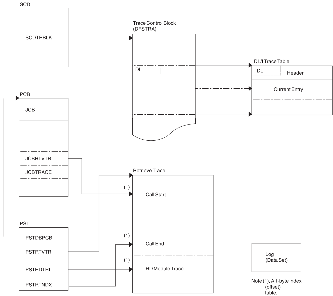
Figure 83. How to Locate the Database Traces
