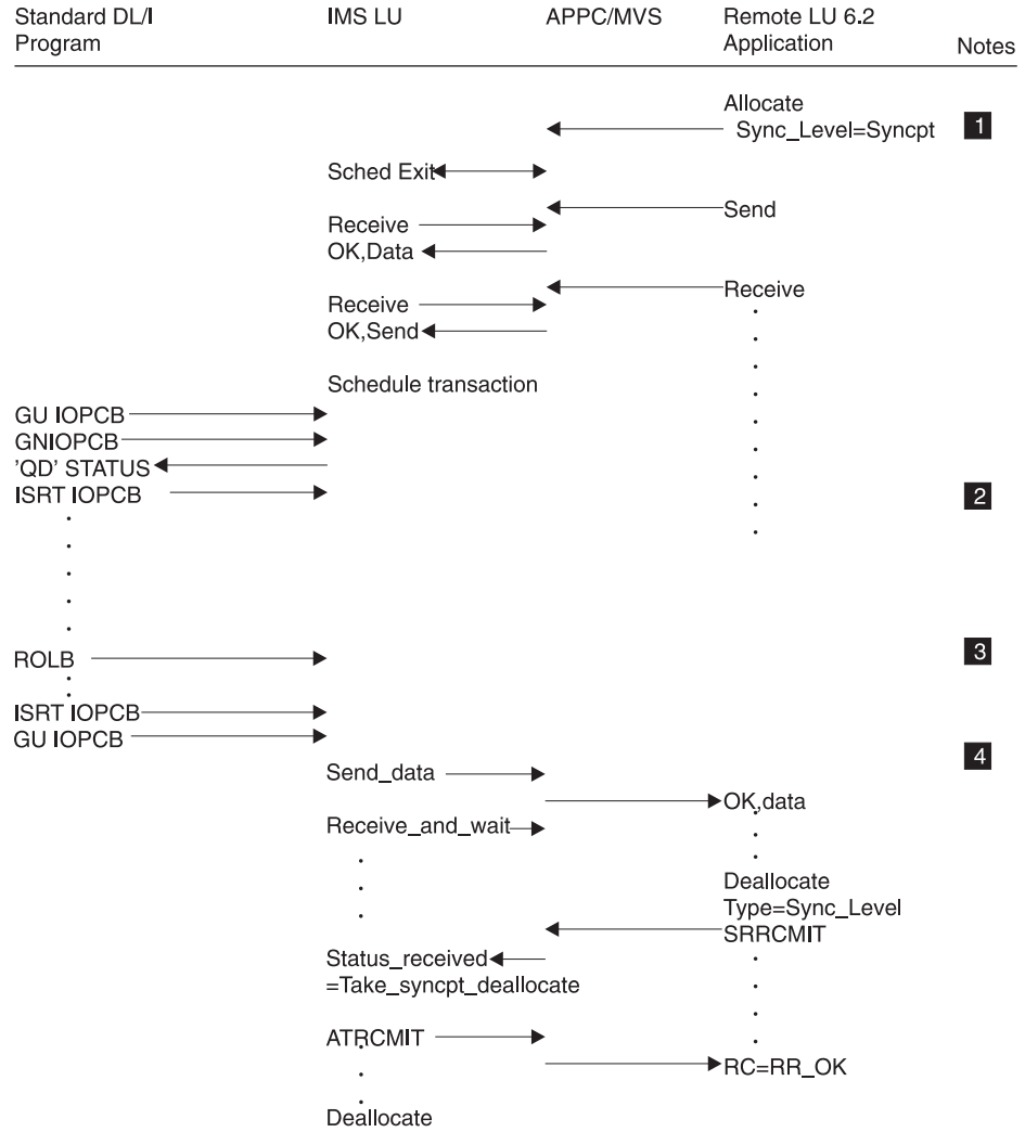
Figure 49. Standard DL/I Program ROLB Scenario When Sync_Level=Syncpt
