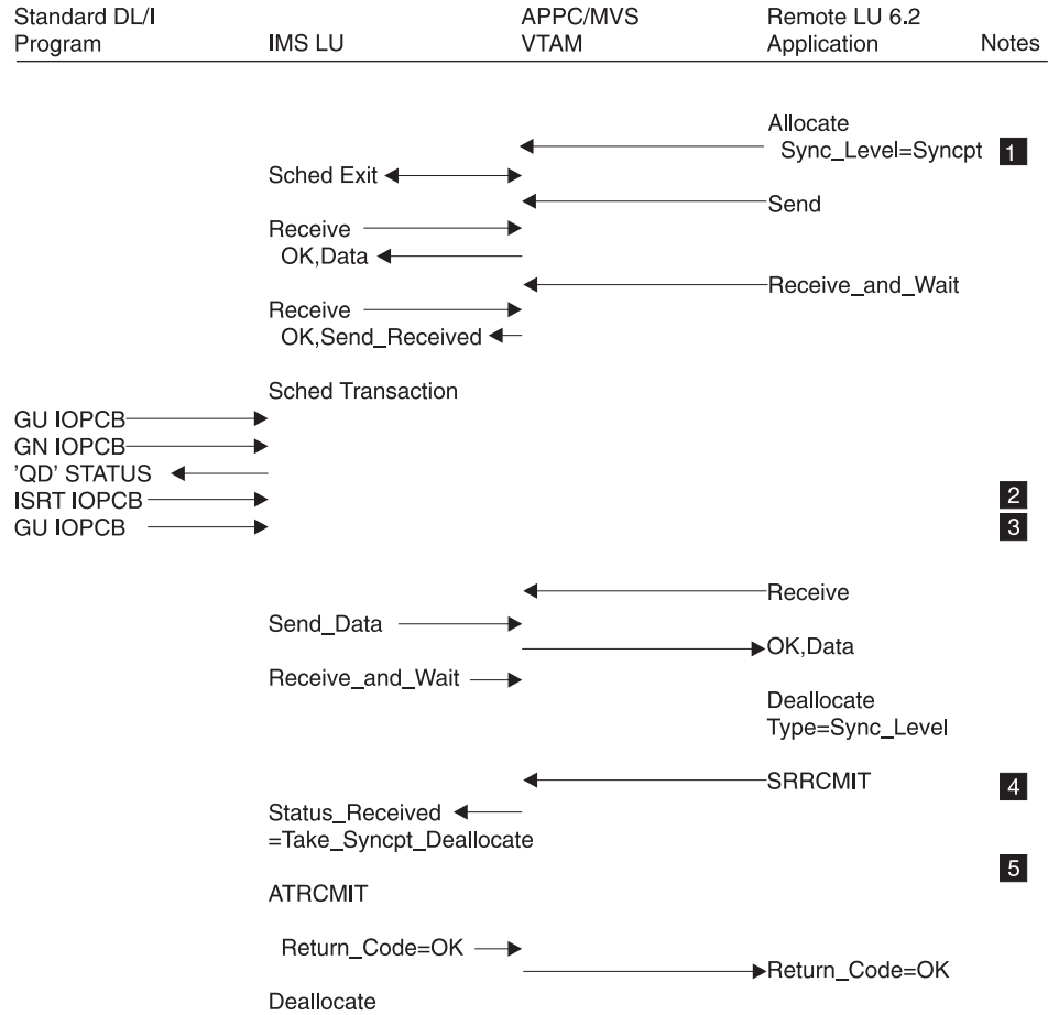
Figure 45. Standard DL/I Program Commit Scenario When Sync_Level=Syncpt
