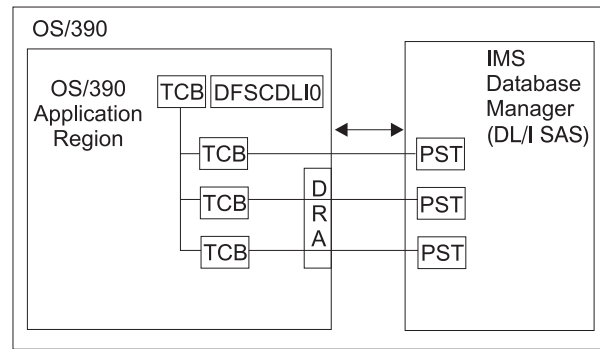
Figure 52. DRA Uses One TCB per Thread
