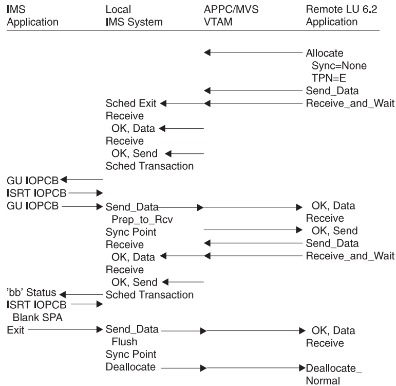
Figure 36. Flow of a Local IMS Conversational Transaction When Sync_level=None
