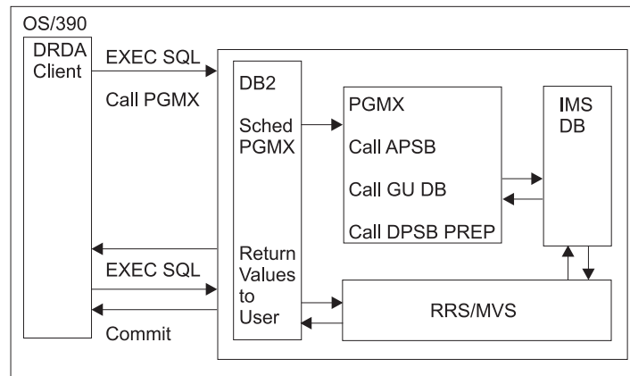
Figure 54. DB2 Stored Procedures Relationships
