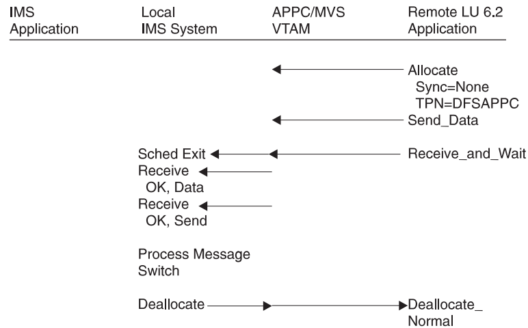
Figure 39. Flow of a Message Switch When Sync_level=None
