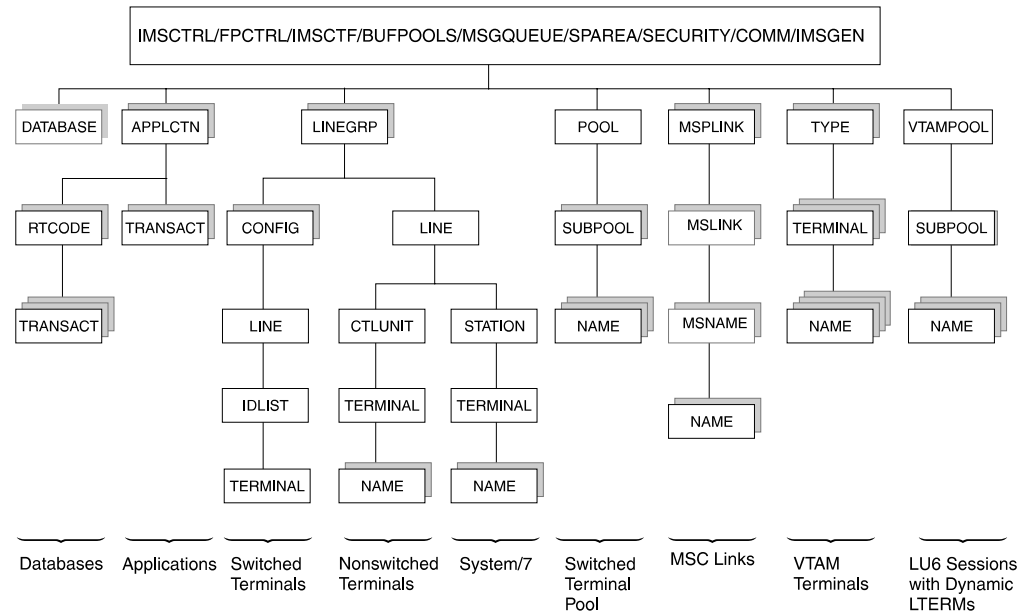
Figure 3. Hierarchy of Stage 1 System Definition Macros
