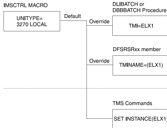
Figure 2. Specifying the Transport Manager Instance (TMI) Name for RSR
