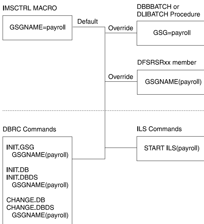
Figure 1. Specifying the Global Service Group (GSG) Name for RSR
