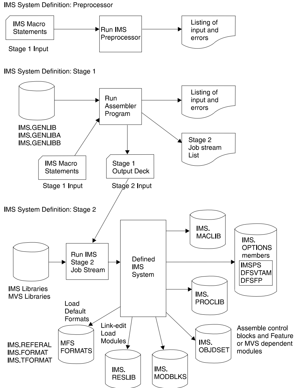
Figure 4. Summary of the Two Stages of System Definition Processing
