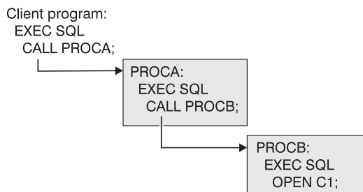
Figure 39. Nested CALL statements
