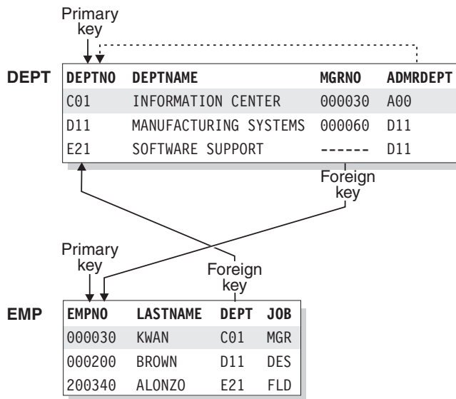
Figure 4. Referential integrity of DEPT and EMP tables
