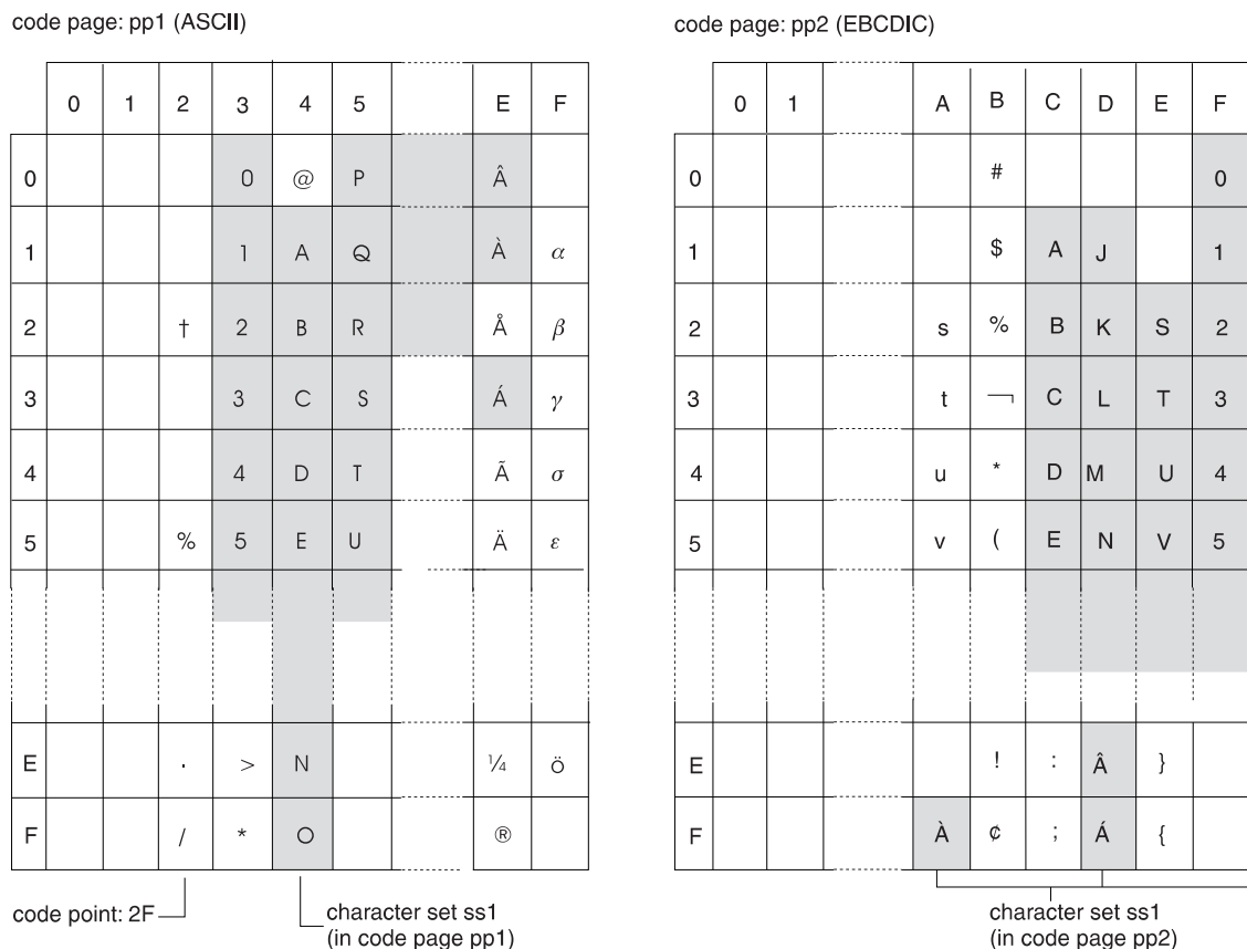
Figure 16. Code page mappings for character set ss1 in ASCII and EBCDIC
