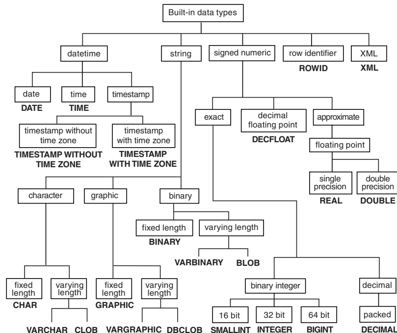
Figure 21. Built-in data types supported by DB2
