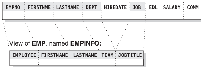
Figure 6. A view of the EMP table
