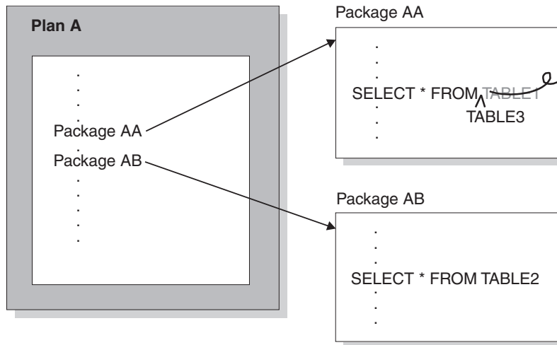
Figure 15. Application plan and packages
