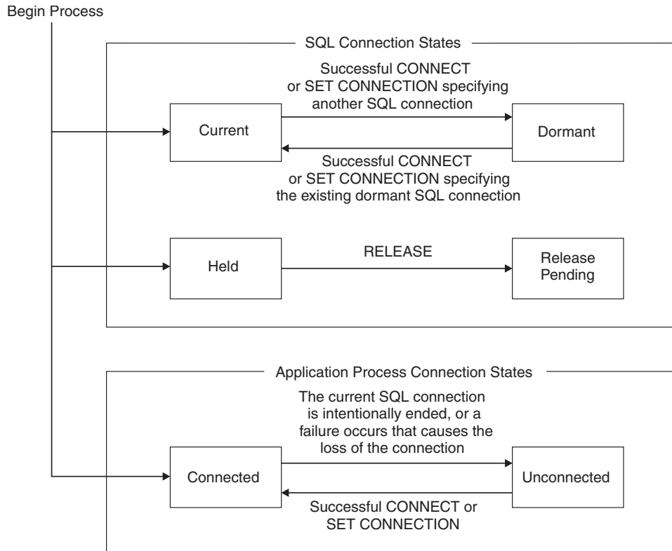
Figure 19. State transitions for an SQL connection and an application process connection in a distributed unit of work
