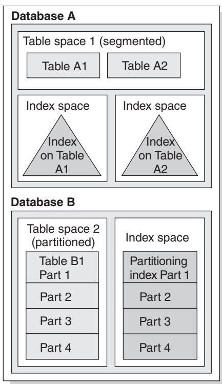
Figure 11. Data structures in a DB2 database
