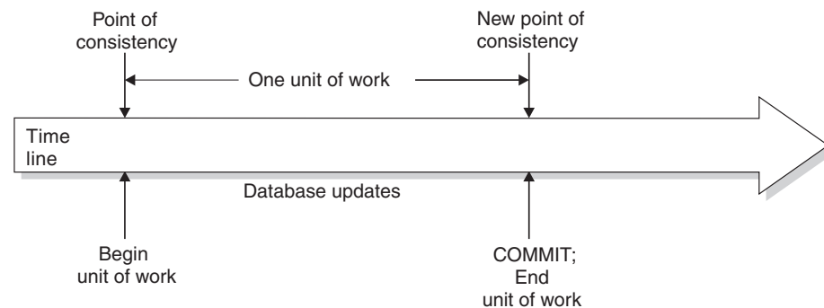
Figure 12. Unit of work with a commit operation
