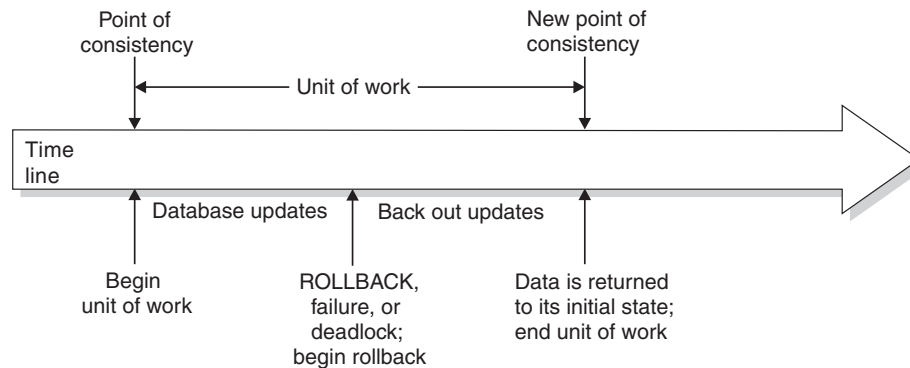
Figure 13. Rolling back all changes from a unit of work
