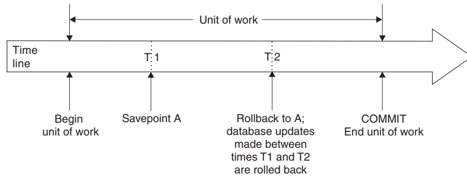
Figure 14. Rolling back changes to a savepoint within a unit of work
