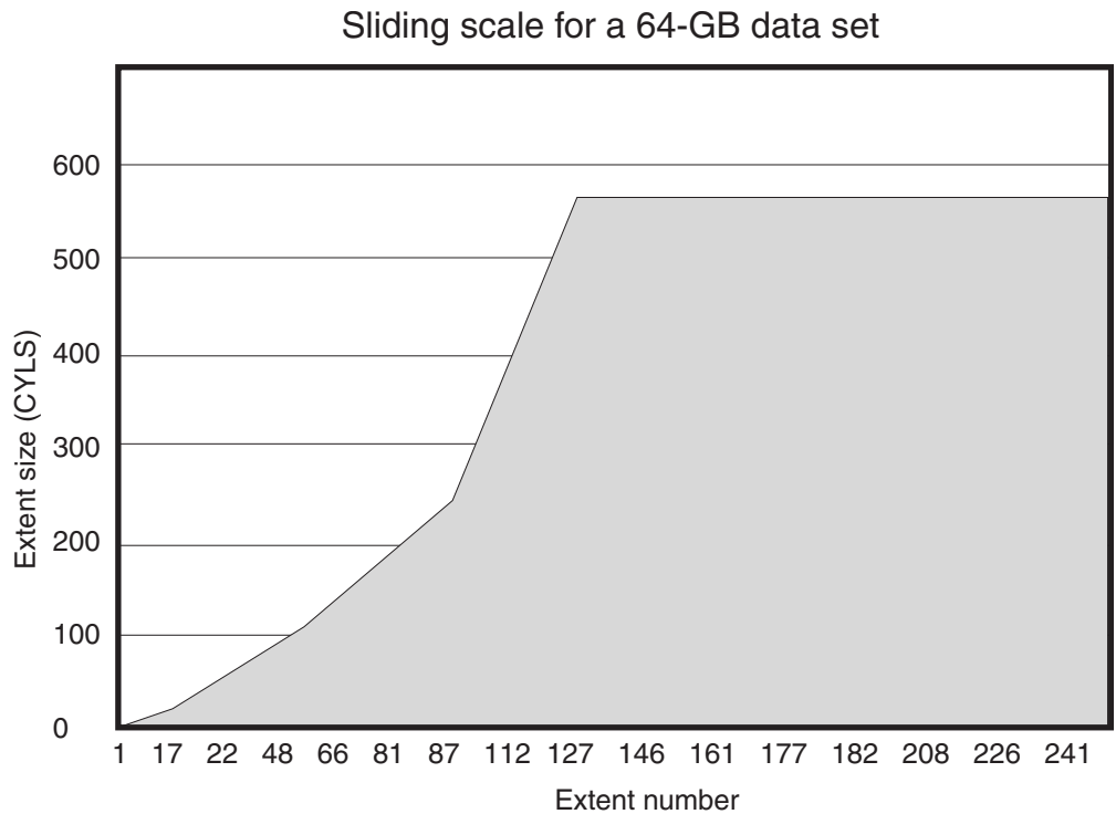
Figure 40. Sliding scale allocation of secondary extents for a 64 GB data set
