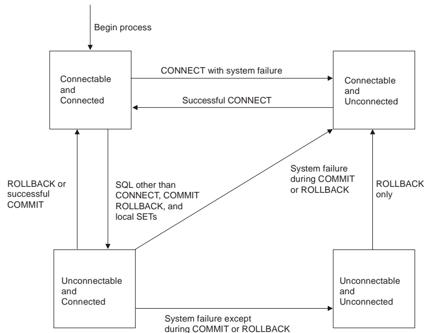
Figure 20. State transitions for an application process connection in a remote unit of work
