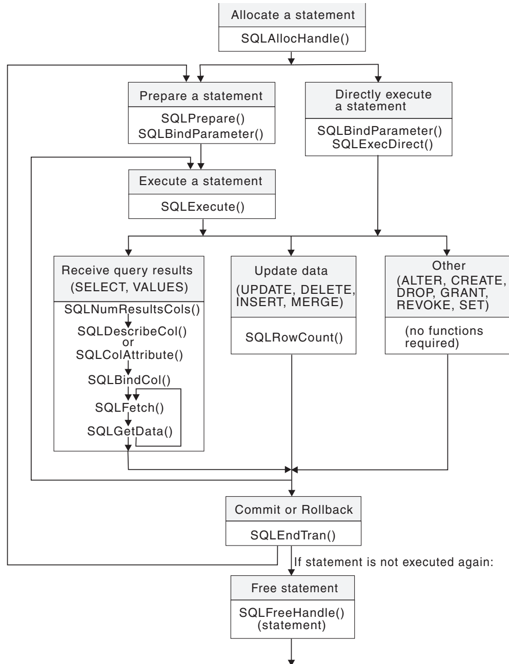
Figure 4. Transaction processing
