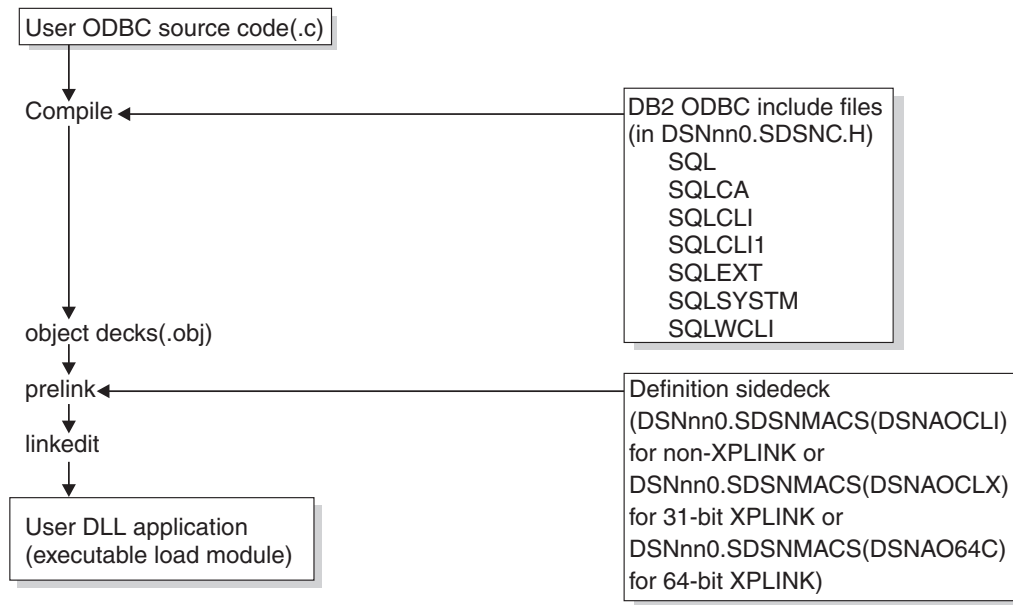
Figure 8. DB2 ODBC program preparation
