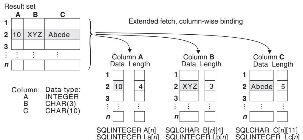
Figure 46. Column-wise binding
