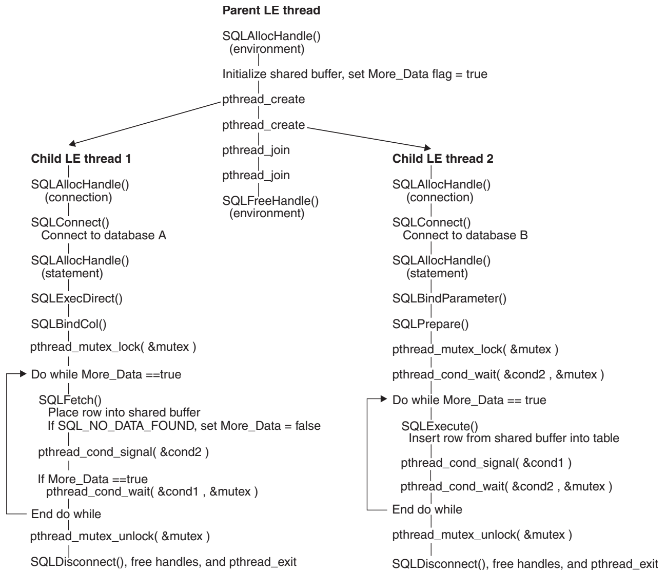
Figure 61. Multithreaded application
