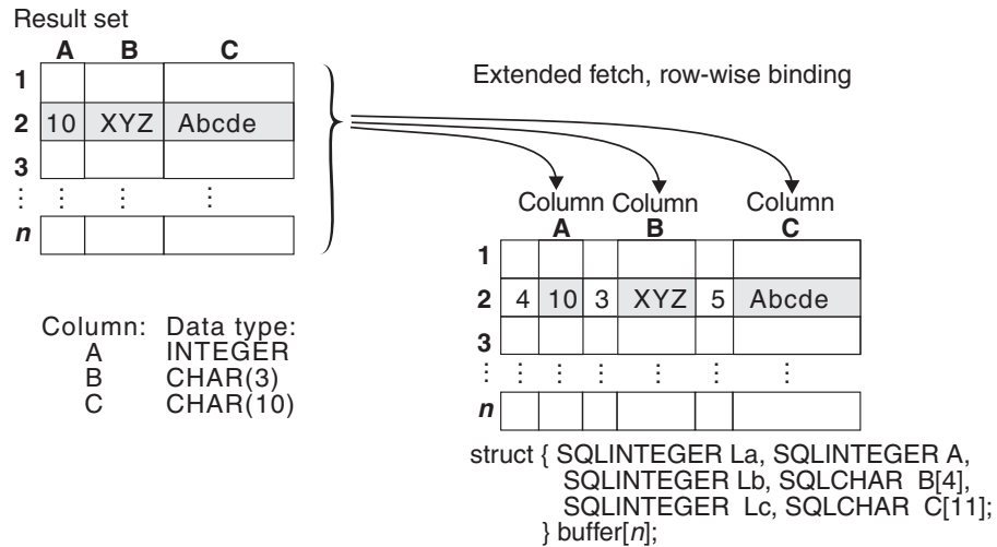
Figure 47. Row-wise binding
