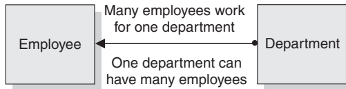
Figure 61. Assigning many-to-one facts to an entity
