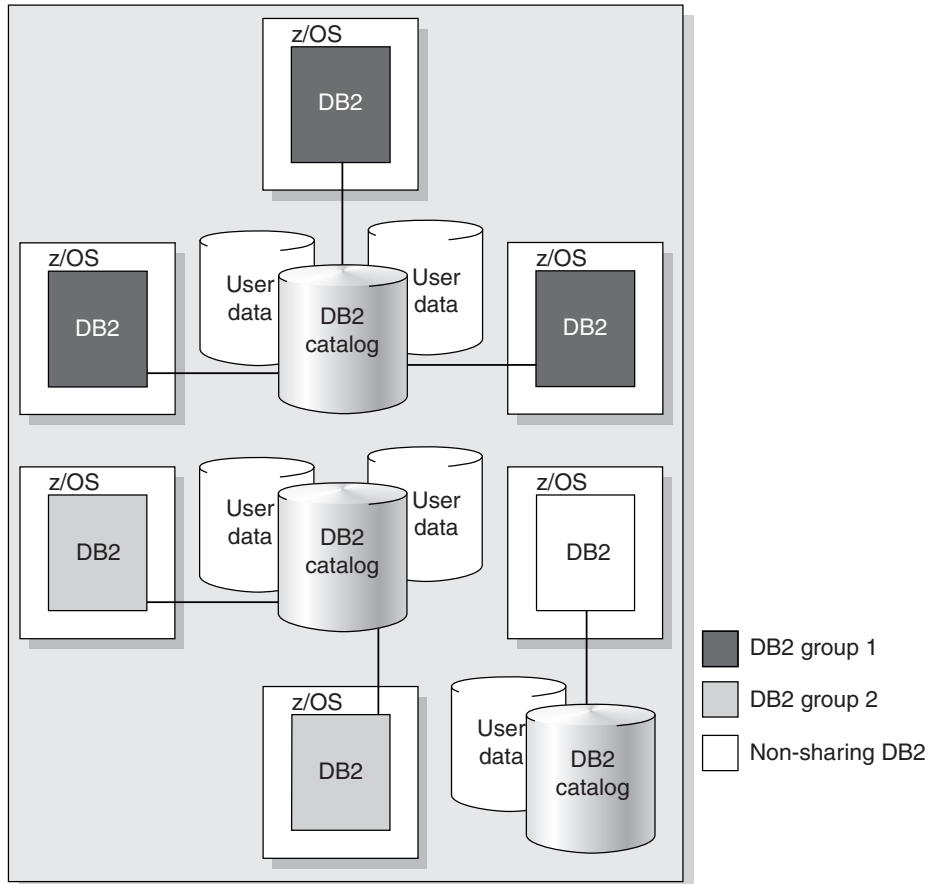
Figure 37. A possible configuration of DB2 data sharing groups. Although this example shows one DB2 for each z/OS system, your environment could have more.
