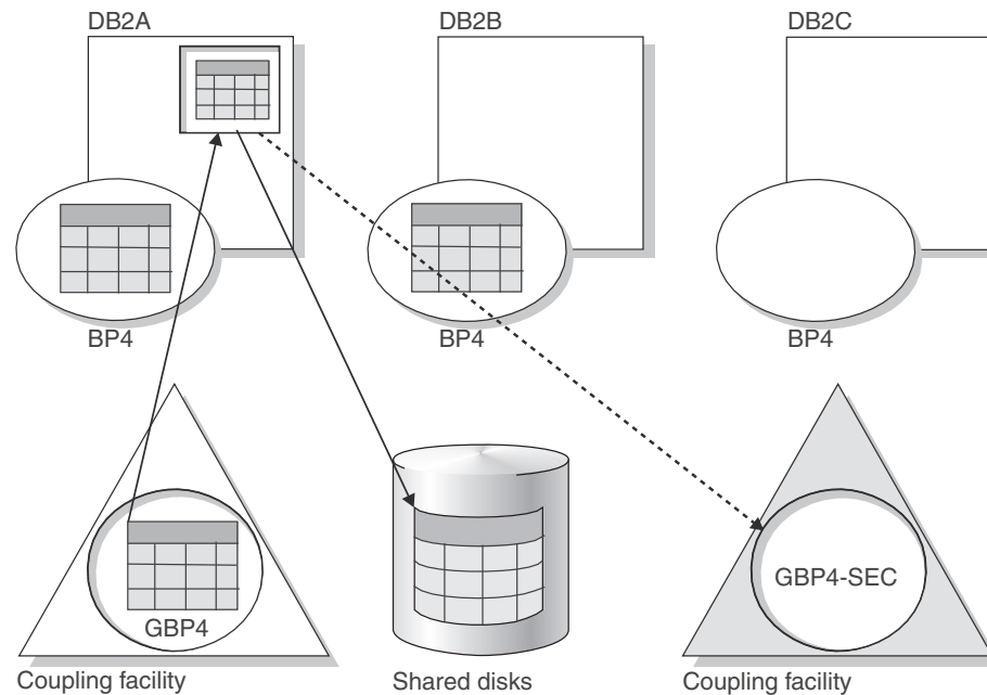
Figure 45. Writing data to disk
