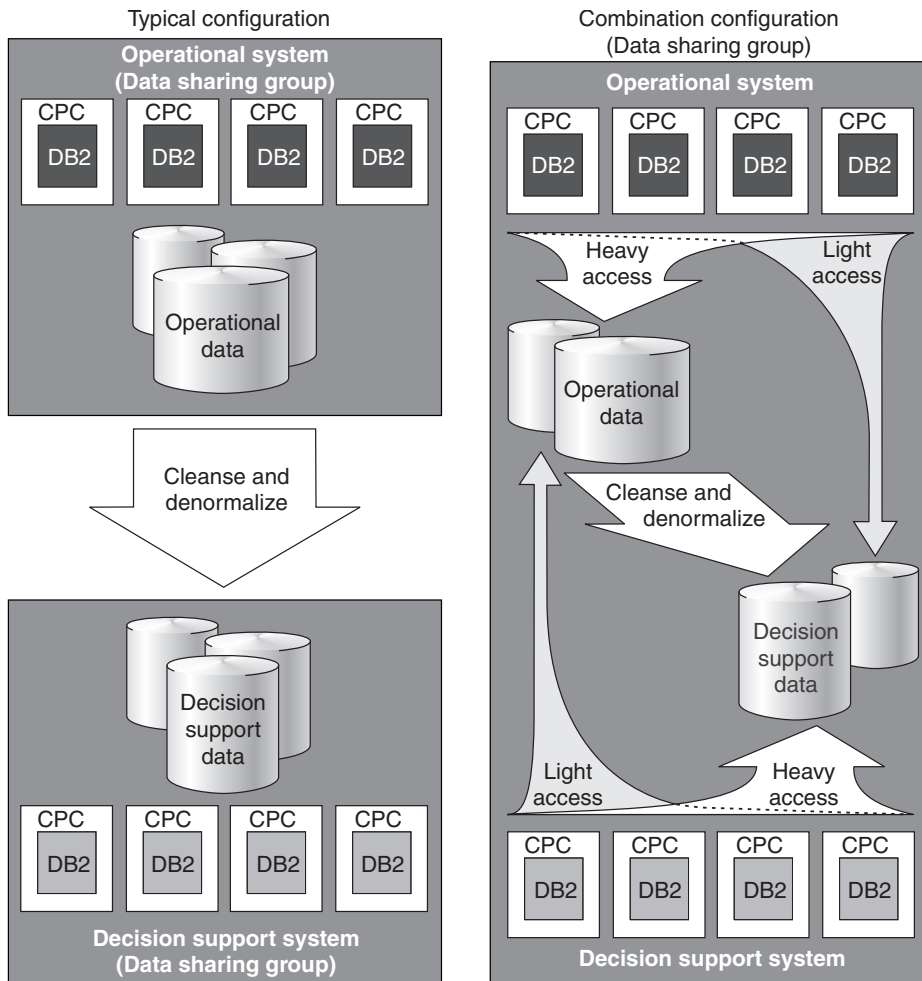
Figure 39. Flexible configurations for decision support. DB2 data sharing lets you configure your systems in the way that works best within your environment.
