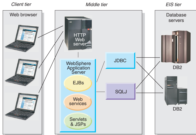
Figure 58. n-tier connectivity with a workstation-based client, two web servers, and different database servers
