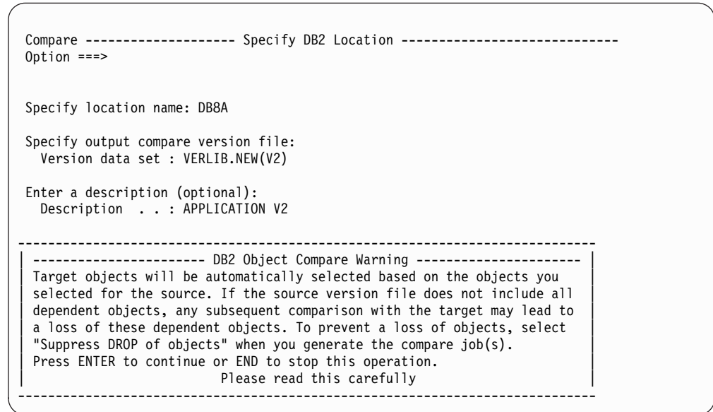
Figure 38. Specify DB2 Location panel (GOC14)
