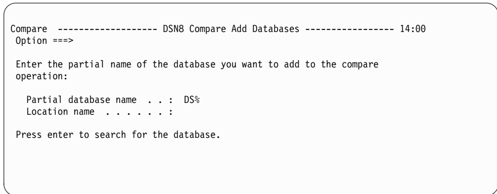
Figure 16. DB2 Compare Add Database panel (GOC1DA)
