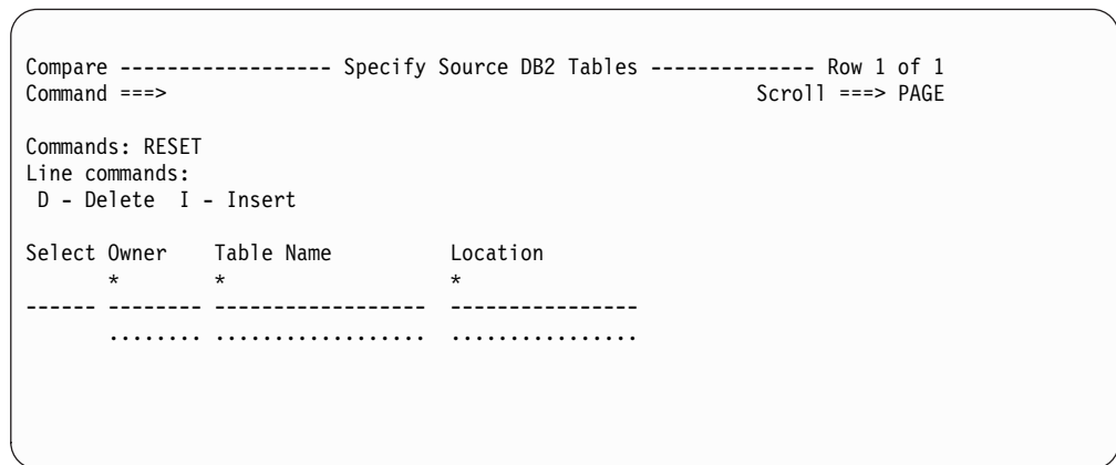
Figure 22. Specify Source DB2 Tables panel (GOC1T)
