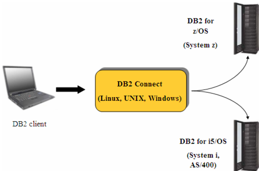
Figure 2.2 – DB2 Connect
