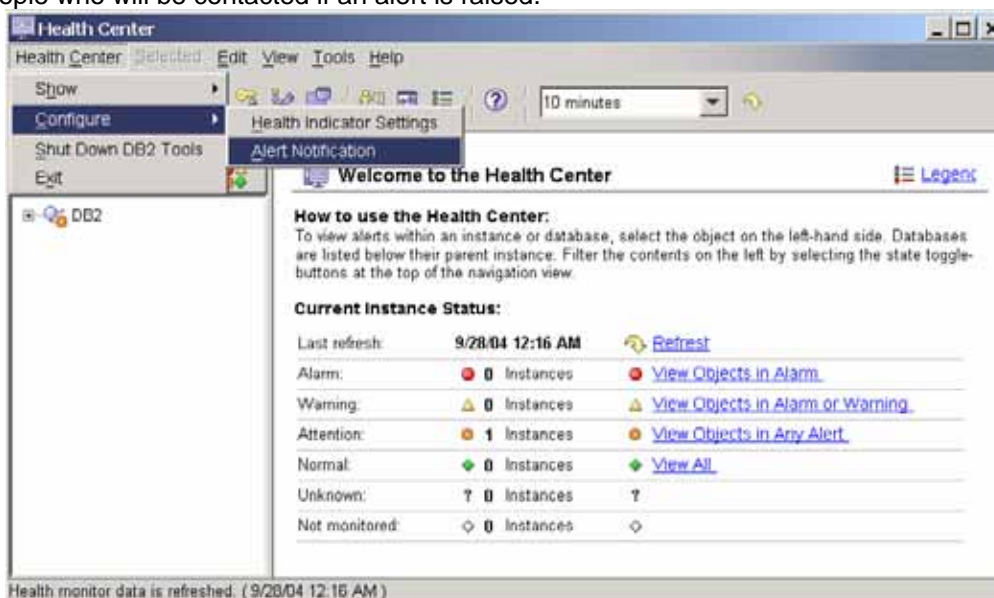
Figure 5.21 – Alert Notification
