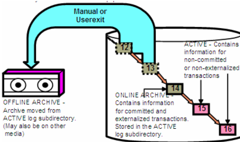
Figure 11.3 – Archival logging
