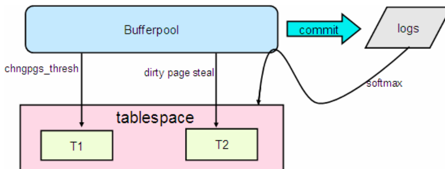
Figure 11.1 – Database logging
