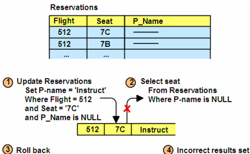
Figure 13.5 – Uncommitted Read
