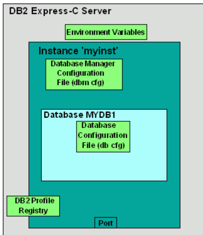
Figure 4.12 – DB2 Configuration
