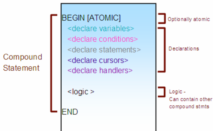
Figure 14.7 – Compound statements
