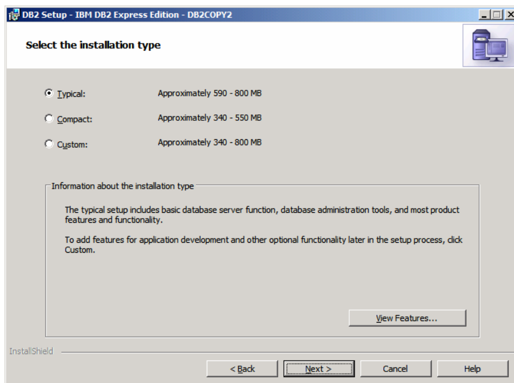
Figure 3.2 – Installation types
