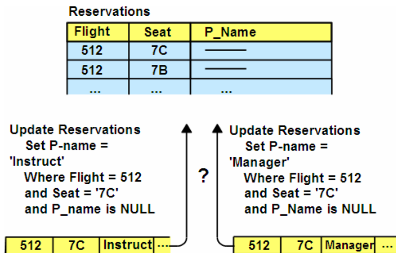
Figure 13.4 – Lost Update
