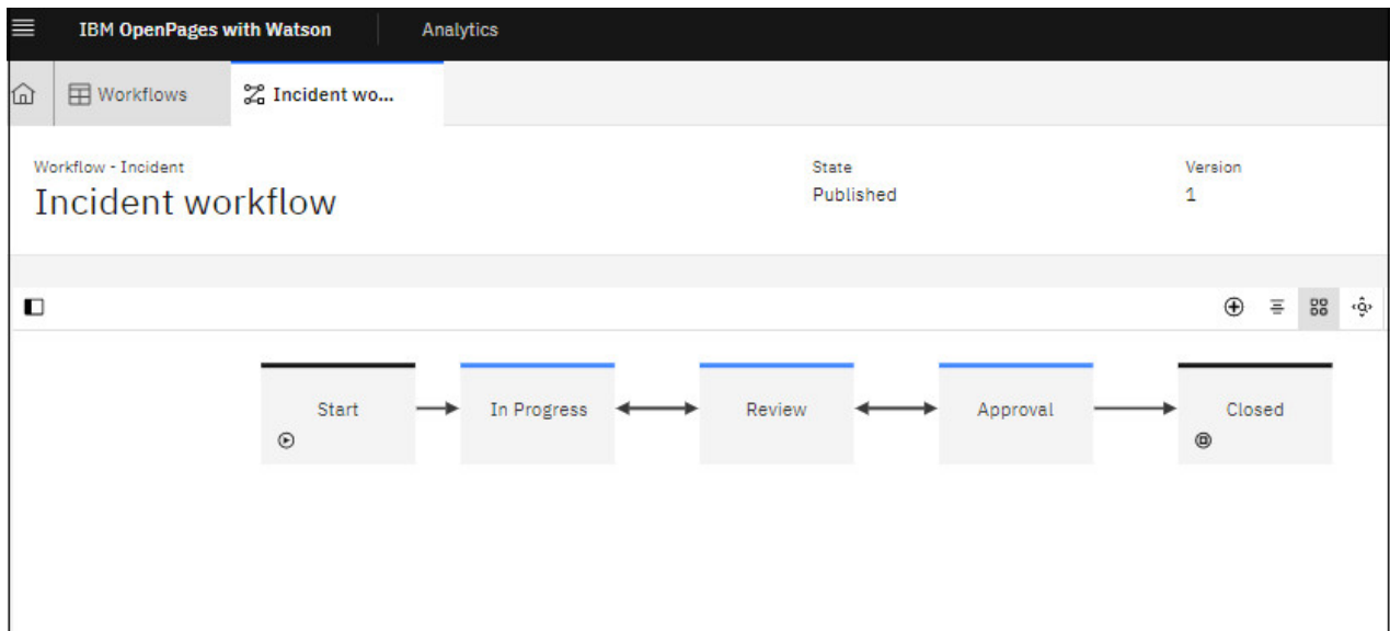
Figure 6. Incident workflow
