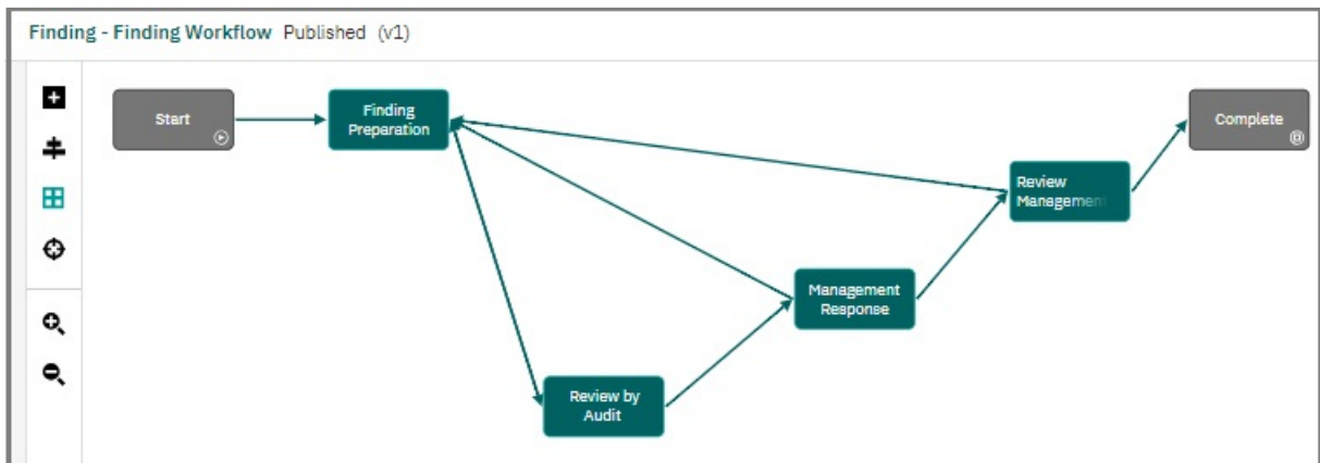
Figure 4. Finding workflow
