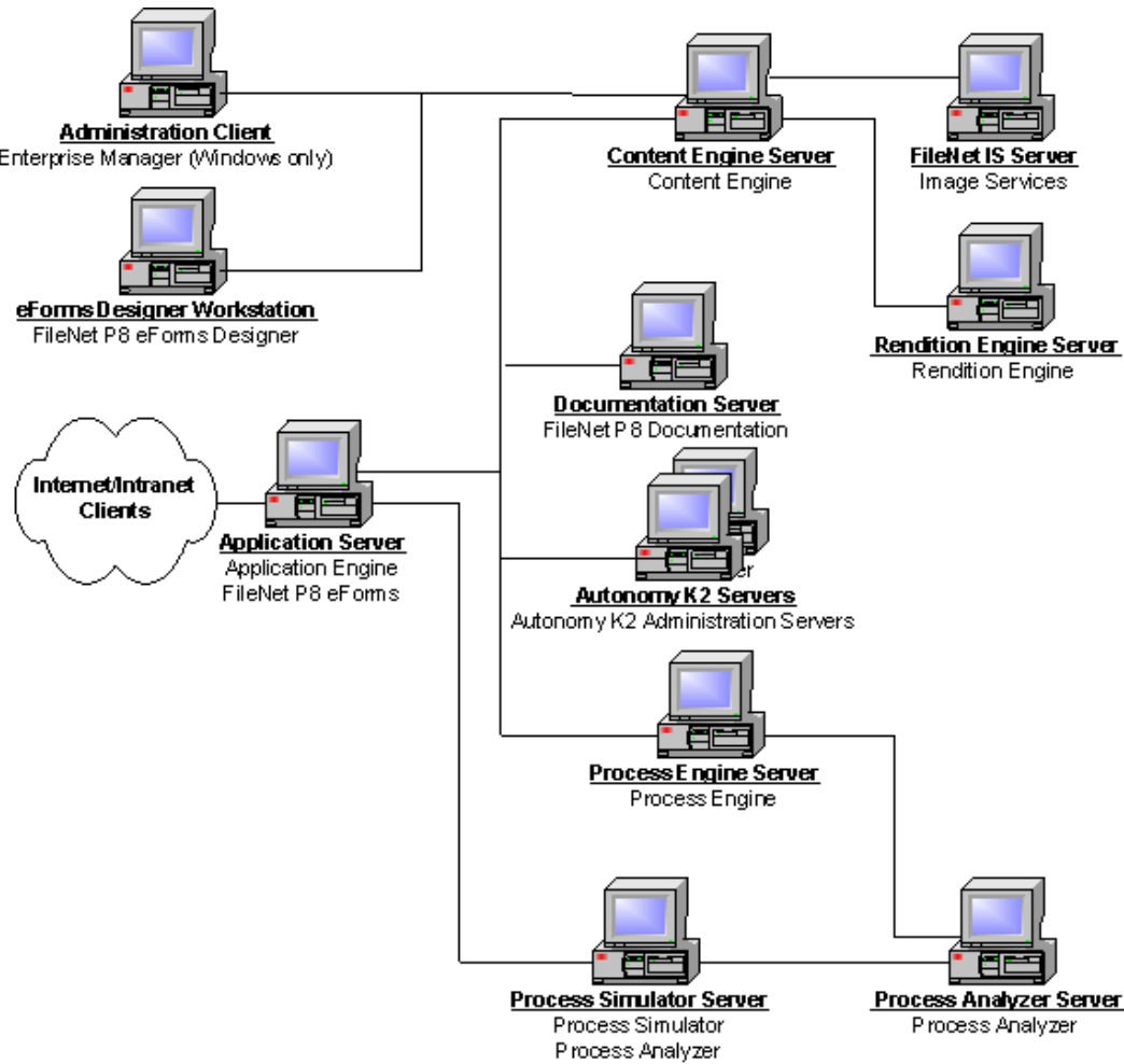
Figure 2: Baseline Configuration With Optional Components
