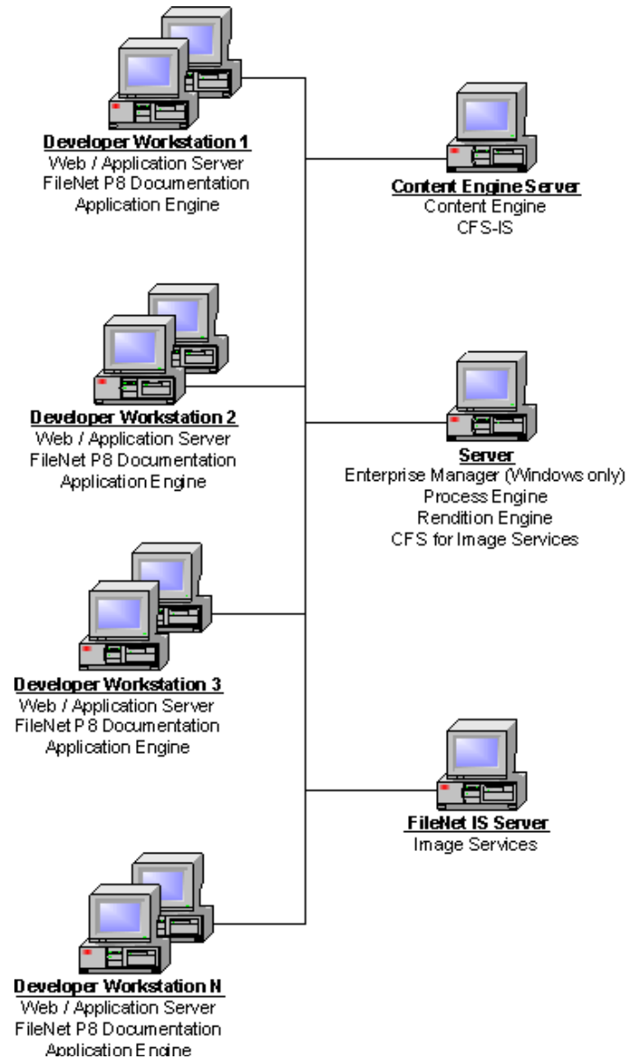
Figure 3: Developer Configuration
