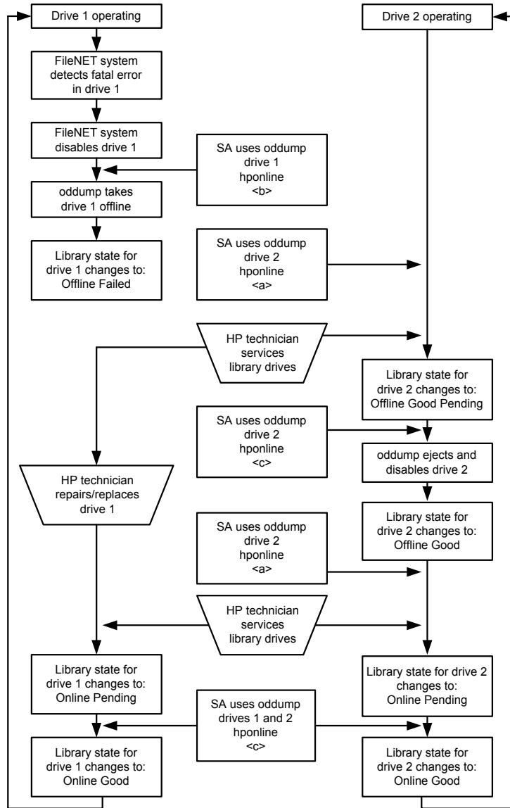
Drive State Diagram for Dual-Drive Bracket Storage Library
