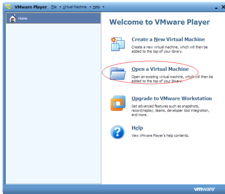
VMware Player
