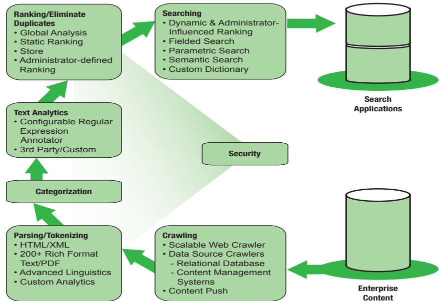
Figure 4. The flow of content through the OmniFind Enterprise Edition system.
