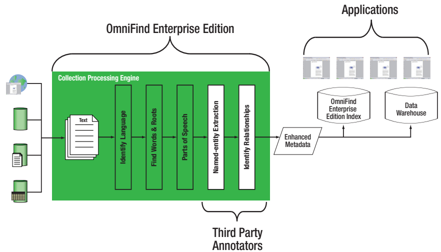
Figure 14. OmniFind Enterprise Edition is the first commercially available UIMA-based platform for processing text-based information.
