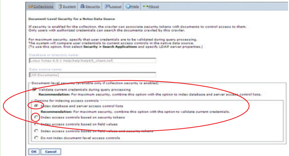
Figure 8. If the option to validate security credentials is selected, OmniFind Enterprise Edition will consult the Lotus Notes/Domino Access Control Lists (ACLs) during query processing to make sure the user still has access to the specified documents.
