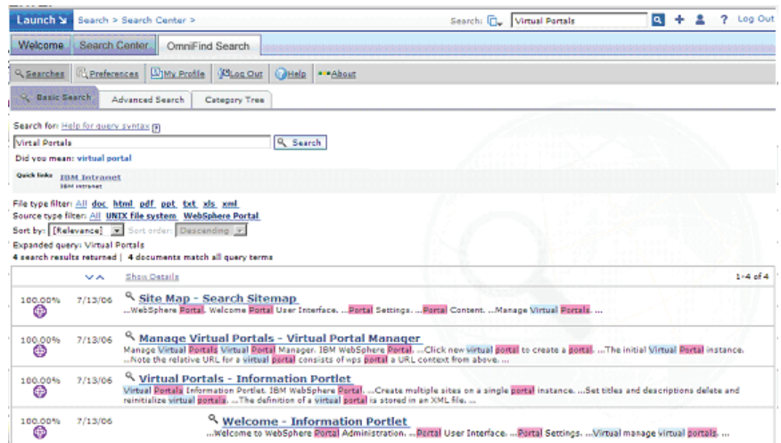
Figure 11. The OmniFind Enterprise Edition search portlet exposes all of the advanced search functionality available in OmniFind Enterprise Edition directly through the portal.
