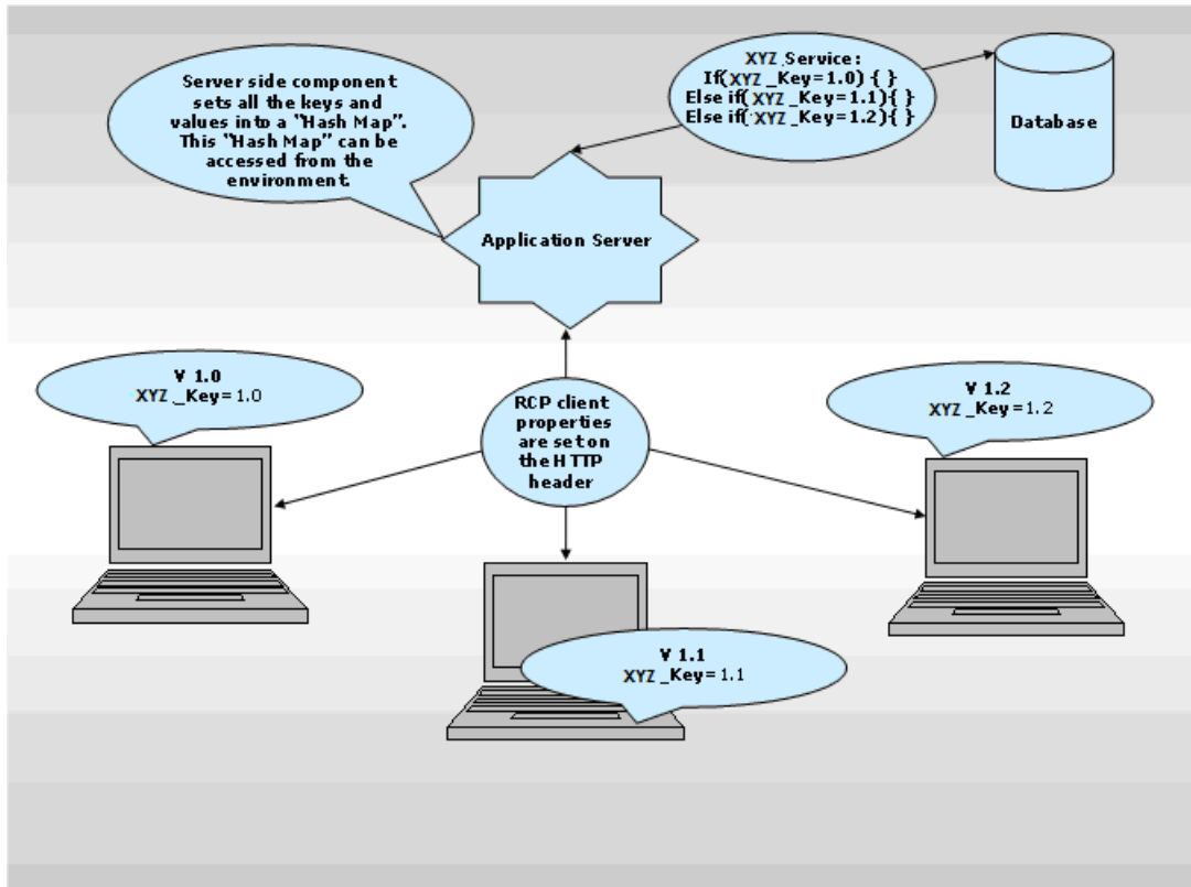
Figure 2–8 Layout of the client-server communication process
