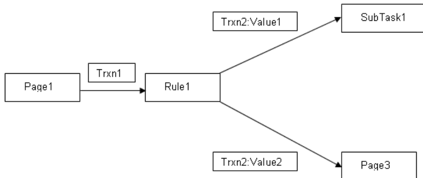
Figure 6–2 Sample Wizard Flow
