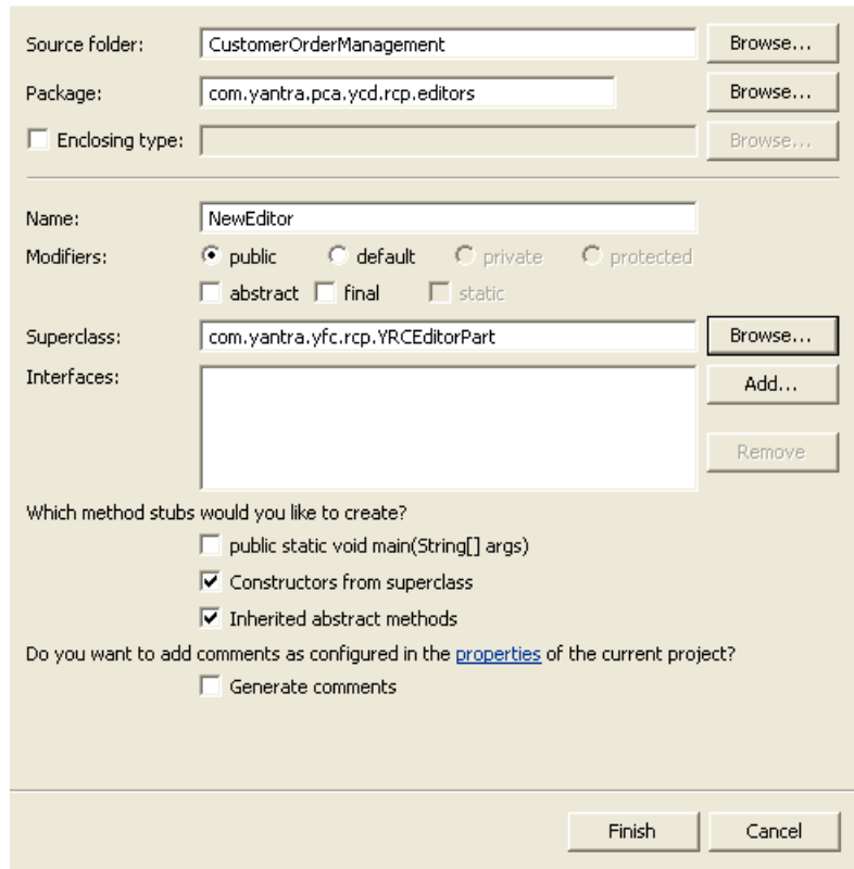
Figure 7–12 Java Attribute Editor Window
