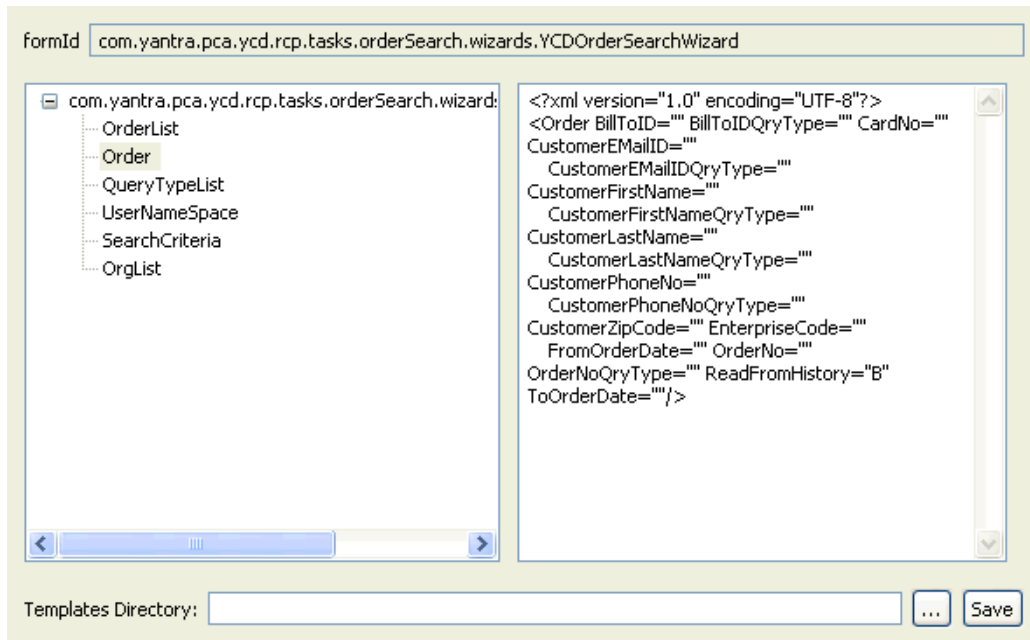
Figure 0–2 The Screen Models Window
